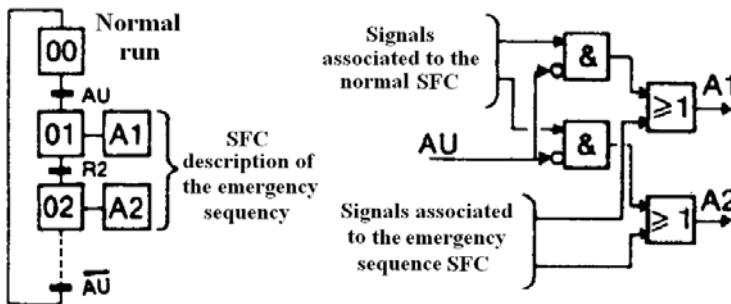
Fig. 17. Introduction of an emergency sequence
