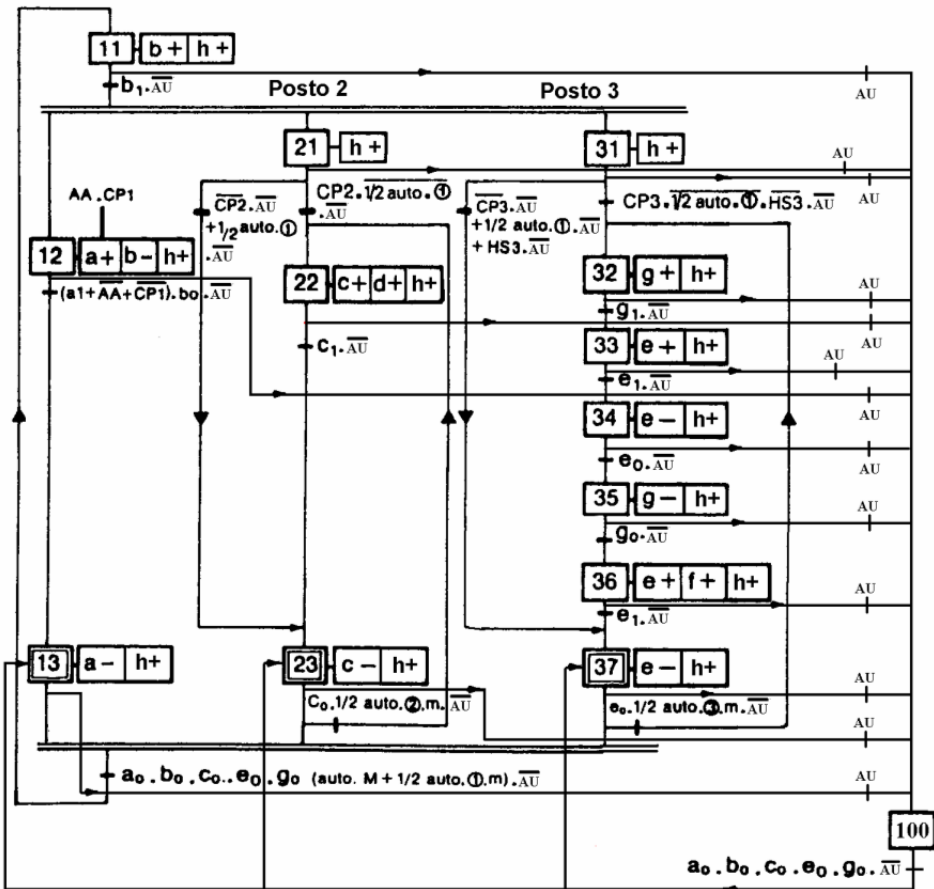
Fig. 18. Total SFC controller specification with emergence sequence
