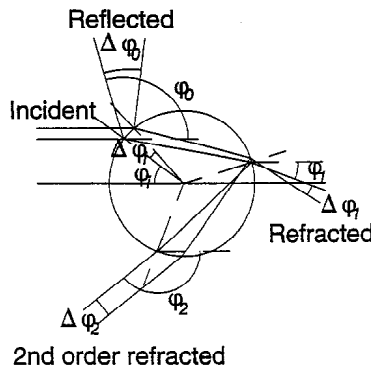
Figure 12. Light scattering modes from a spherical particle
