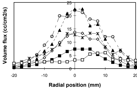
Figure 6. Mass flux as a function of ALR
