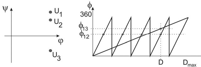
Figure 13. Removing the 2\pi ambiguity
