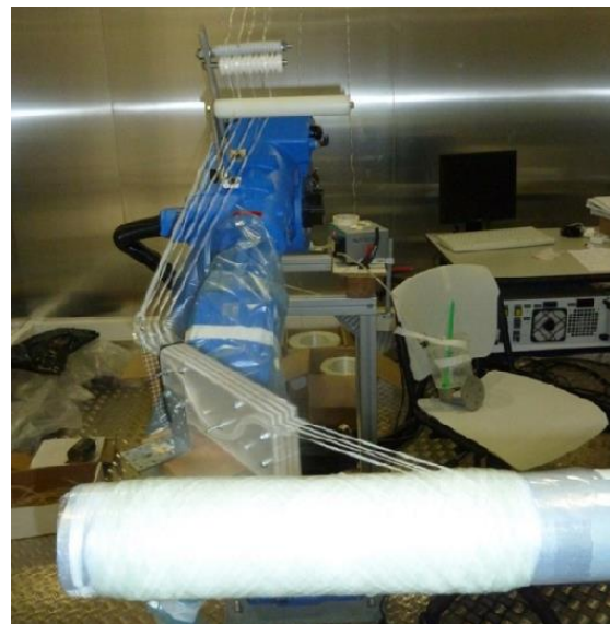
Figure 6. The filament winding with four roving.
