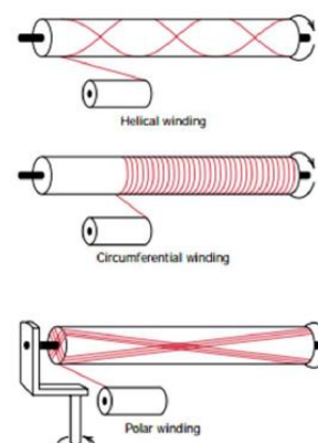
Figure 1. Three different types of winding.
