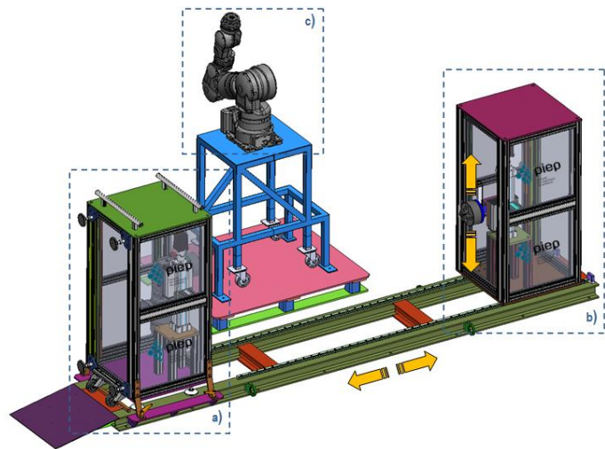
Figure 8. Final filament winding kit.
