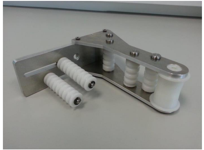
Figure 3. Payout eye used in the dip-resin bath process.
