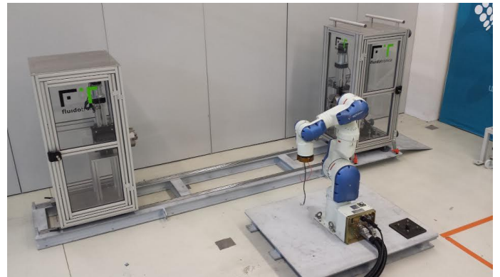
Figure 9. Filament winding kit assembly.
