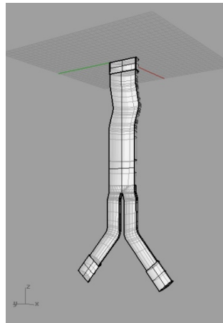
Figure 1. AAA geometry: a) main modeling parameters, b) 3D mechanical model and c) 3D fluidic model.
