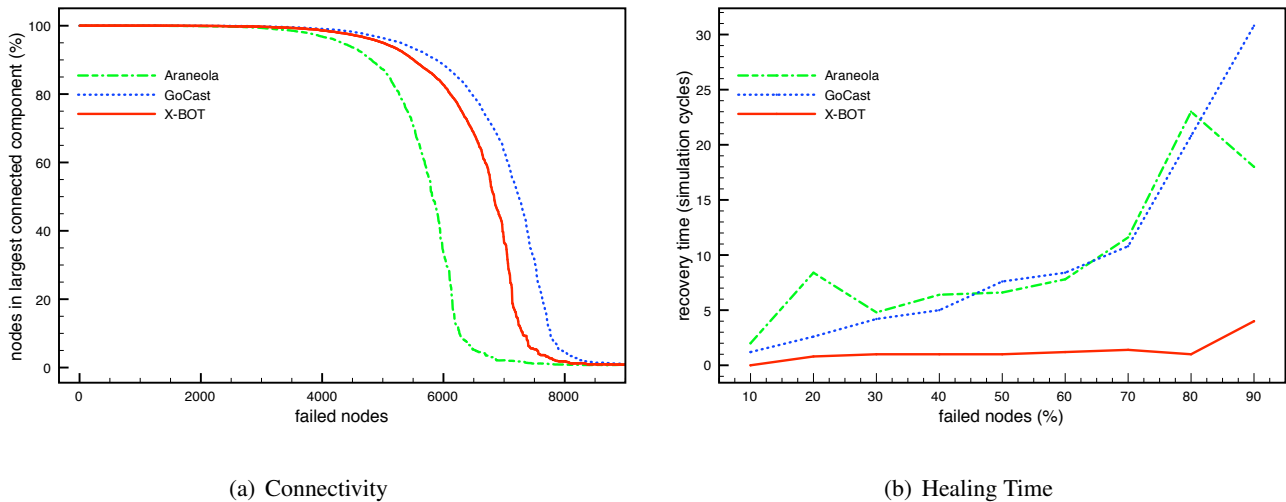
Figure 4. Overlay resilience.
