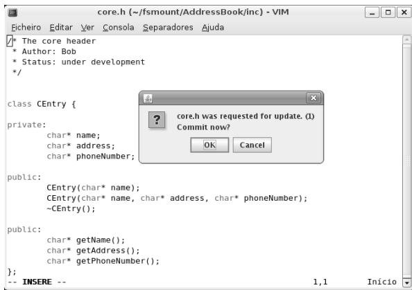
Figure 2. Bob being asked to update his uncommitted version of the file (as a result of Alice’s request). In this case, Bob is using the VIM editor.
