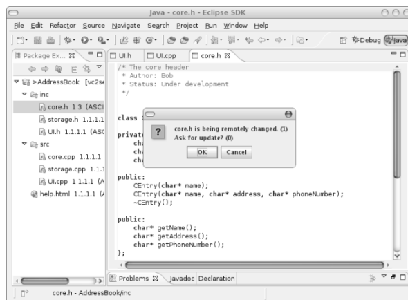
Figure 1. Alice being alerted that the file she wants to access has been modified by some other user. In this case, Alice is using the Eclipse IDE.
