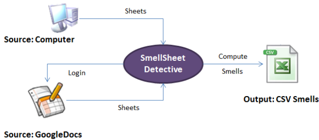
Fig. 1. SmellSheet Detective architecture.
