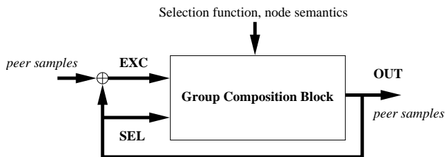
Figure 4: Generic group composition B^2 .
