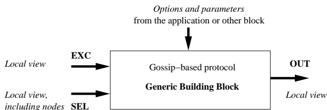
Figure 1: A generic B^2 .
