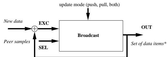
Figure 3: A broadcasting service B^2 .
