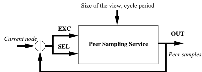
Figure 2: The peer sampling service B^2 .
