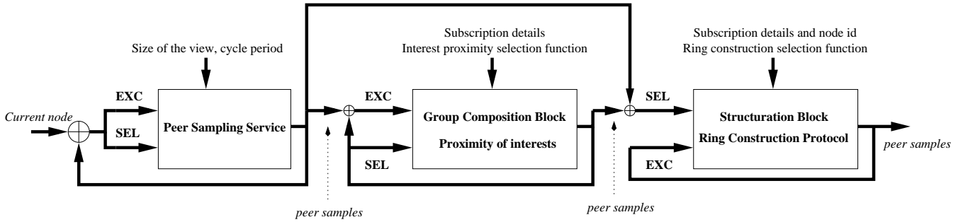
Figure 7: Sub-2-Sub composition of blocks for content-based pub/sub overlay construction [34].
