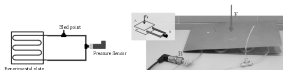
Figure 3. Pressure sensor schematics and construction.
