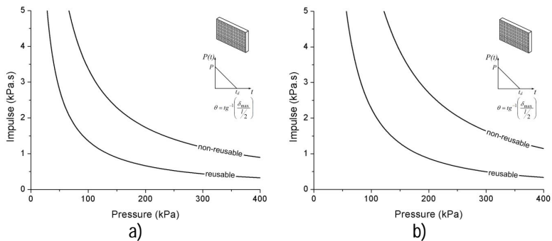
Figure 10. P-I diagram for unreinforced masonry infill panel with minimum grid reinforcement in the plaster: a) 180 mm; b) 230 mm.
