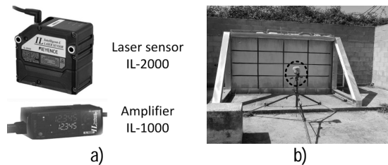
Figure 4. Deflection acquisition: a) laser sensor and amplifier; b) laser mounted in place.
