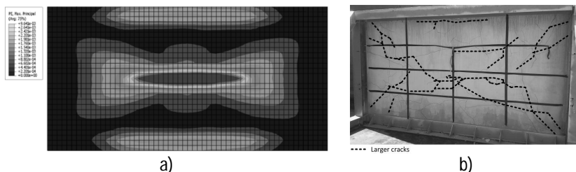
Figure 7. Damage pattern: a) location of the maximum principal plastic strains; b) larger cracks after the test.
