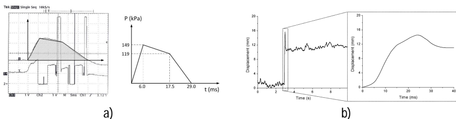
Figure 5. Acquired signals: a) pressure profile; b) displacement profile.
