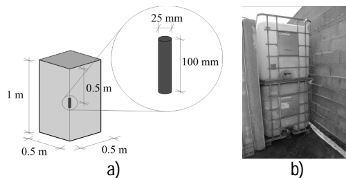
Figure 2. WBWG: a) explosive charge location; b) placing the water container in the final position.
