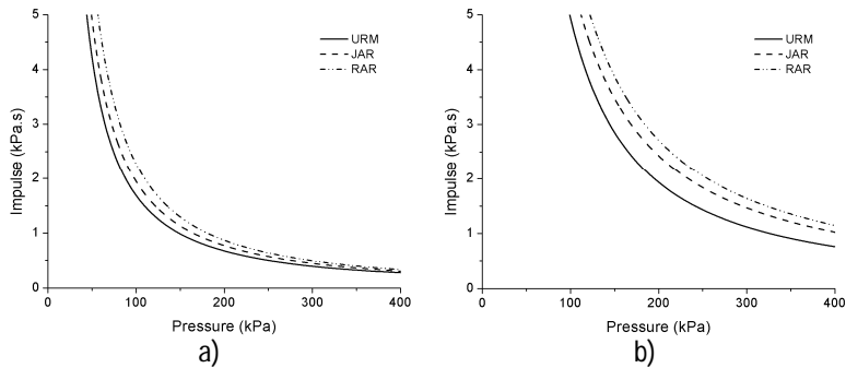
Figure 12. P-I diagrams comparing three solutions for 230 mm: a) reusable stage; b) non-reusable stage.
