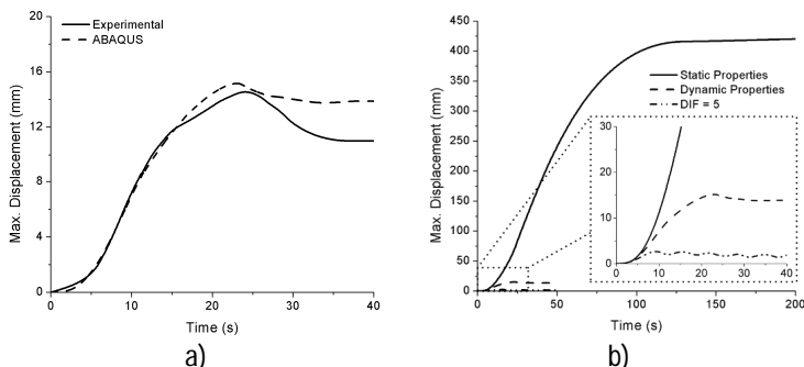
Figure 6. Numerical results: a) Comparison between the numerical and experimental results; b) Influence of the dynamic increase factors on the behaviour of the wall.
