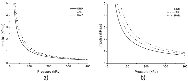
Figure 11. P-I diagrams comparing three solutions for 180 mm: a) reusable stage; b) non-reusable stage.
