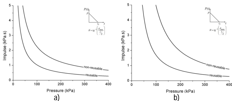
Figure 8. P-I diagram for unreinforced masonry infill panel: a) 180 mm; b) 230 mm.
