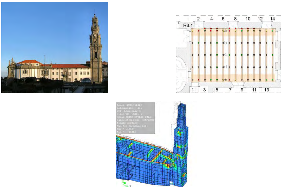
Figure 7 – Details of the Clérigo’s Church in Porto: view (left); deterioration in the main floor (right); FEM model and damage predicted (lower center).
