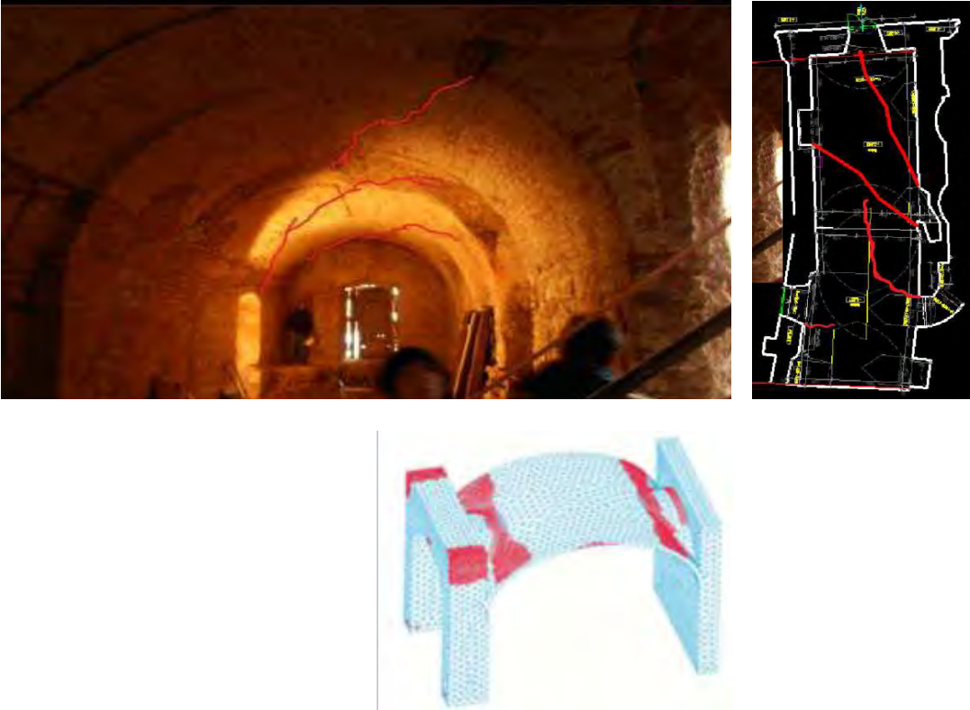
Figure 4 – Interior view of vault (left); crack mapping (right); non-linear analysis of vault to determine crack locations (lower center)
