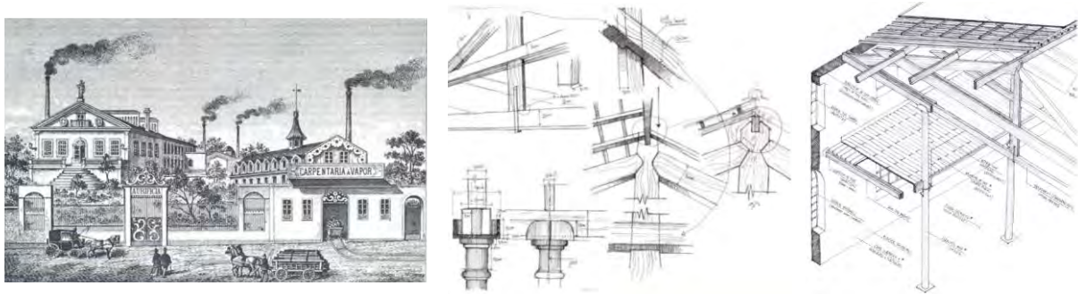
Figure 8 – Details of the Aurificia Company in Porto: old print (left); hand drawings of some of the details (center); summary of the recommended actions (right).
