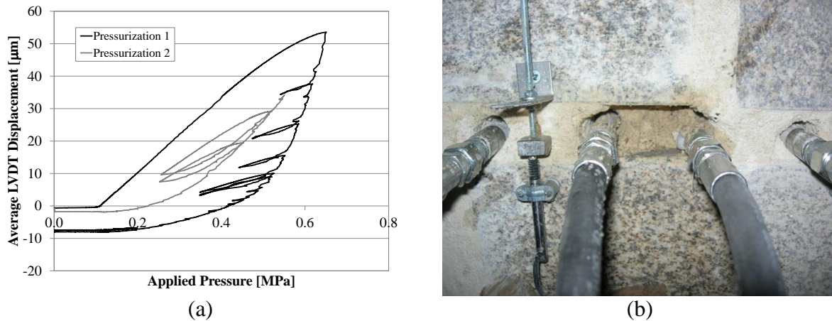
Figure 6 Latex tube-jack pressurization in the 4 th horizontal joint: (a) Applied pressure versus average LVDT displacements; and (b) rupture of a latex tube-jack and damage to the mortar joint during the 2nd pressurization.
