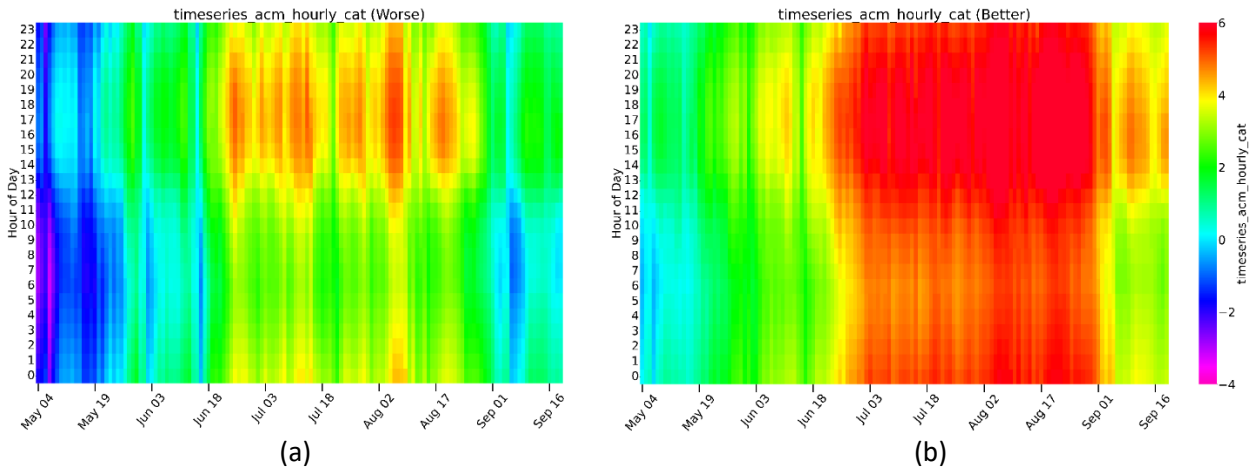
Figure 17: ACM distance from central line carpet plots for Magisterparken A free running season in (a) the less insulated case and (b) the most insulated case
