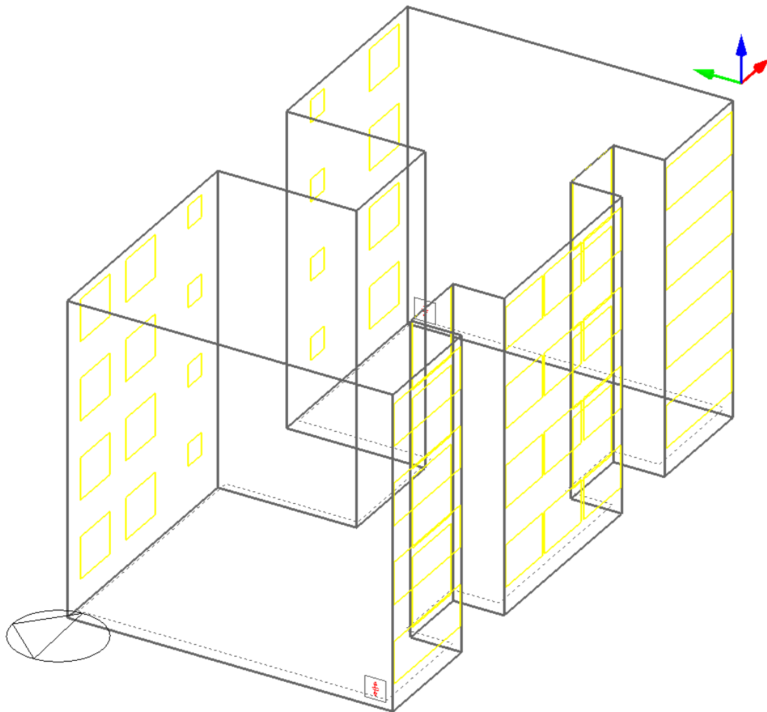
Figure 2 All rooms at all levels are grouped as one single thermal zone for the entire building.
