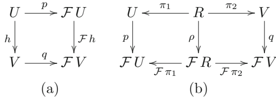
Figure 1. (a) morphism; (b) bisimulation
