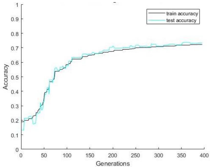
Figure 19b: Training and Validation accuracy of Low-rank GA-CNN (R=5)
