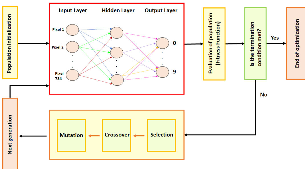
Figure 12: Genetic CNN
