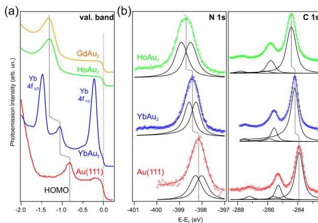
Fig. 5 Photoemission measurements for CuPc/ \text{REAu}_2 samples in comparison to CuPc/Au(111). 75 (a) Valence bands measured on CuPc ML grown on \text{GdAu}_2 , \text{HoAu}_2 and \text{YbAu}_2 MLs. For comparison the valence band of 1 ML of CuPc/Au(111) is given. ( h\nu = 44 \text{ eV} and 50 \text{ eV} , \theta = (20 \pm 7)^\circ for Au(111) and \text{YbAu}_2 and h\nu = 21.22 \text{ eV} and \theta = (50 \pm 7)^\circ for \text{HoAu}_2 and \text{GdAu}_2 substrates, respectively.) (b) N 1s and C 1s core levels of 1 ML CuPc grown on Au(111), \text{HoAu}_2 and \text{YbAu}_2 ( h\nu = 520 \text{ eV} and 390 \text{ eV} , \theta = (0 \pm 7)^\circ ).
