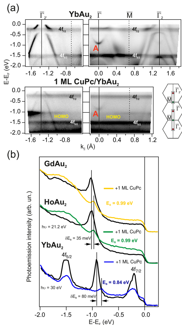
Fig. 4 Representative ARPES band structure of \text{REAu}_2 surfaces compounds before and after CuPc adsorption. (a) Photoemission intensity mapping taken along the indicated \bar{\Gamma}\bar{M} directions of \text{YbAu}_2 (top) and 1 ML CuPc on \text{YbAu}_2 . The non-dispersing HOMO levels of CuPc add to the substrate bands after adsorption ( h\nu = 30 \text{ eV} ). (b) Upshift of the A band upon adsorption of 1 ML of CuPc on \text{YbAu}_2 , \text{HoAu}_2 and \text{GdAu}_2 . The largest shift has been detected in the \text{YbAu}_2 surface compound ( \theta = 0 , h\nu = 30 \text{ eV} [ \text{YbAu}_2 ], 21.2 \text{ eV} [other]).
