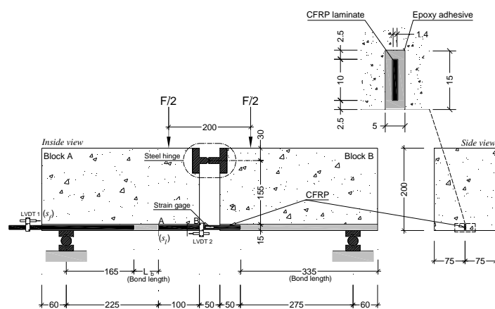
Figure 3: Beam pullout specimens: geometry and test configuration. Note: all units in [mm].
