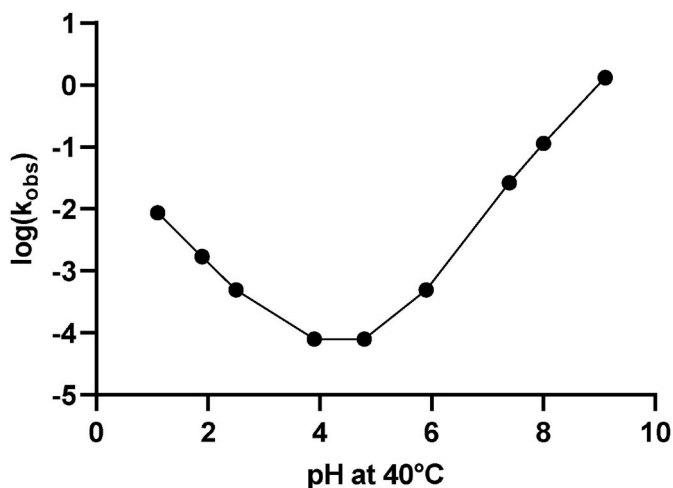
Fig. 3. pH rate ( k_{obs} h -1 ) profile for difluprednate in 5% (w/v) HP \beta CD solution at 40 °C.
