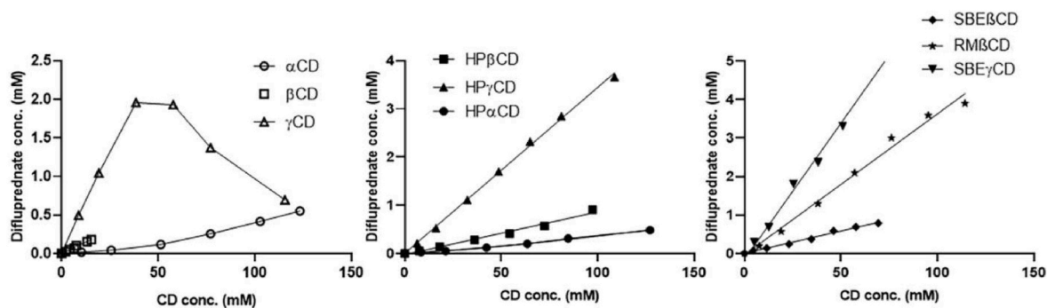
Fig. 4. Phase-solubility diagrams of difluprednate in CD in pure water at room temperature (pH about 5). Each point represents the mean of triplicate experiments. Key: (○) \alpha CD; (□) \beta CD; (△) \gamma CD; (■) HP \beta CD; (●) HP \alpha CD; (▲) HP \gamma CD; (*) RM \beta CD; (▼) SBE \gamma CD and (◆) SBE \beta CD.
