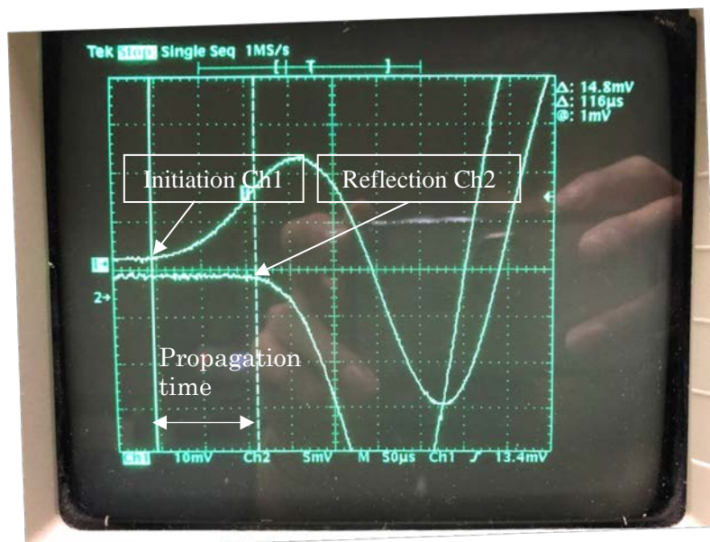
Figure 4. Example of elastic wave measurement in concrete pile Time 50\mu\text{s}/\text{div} . Ch1 10\text{mV}/\text{div} . Ch2 5\text{mV}/\text{div} .
