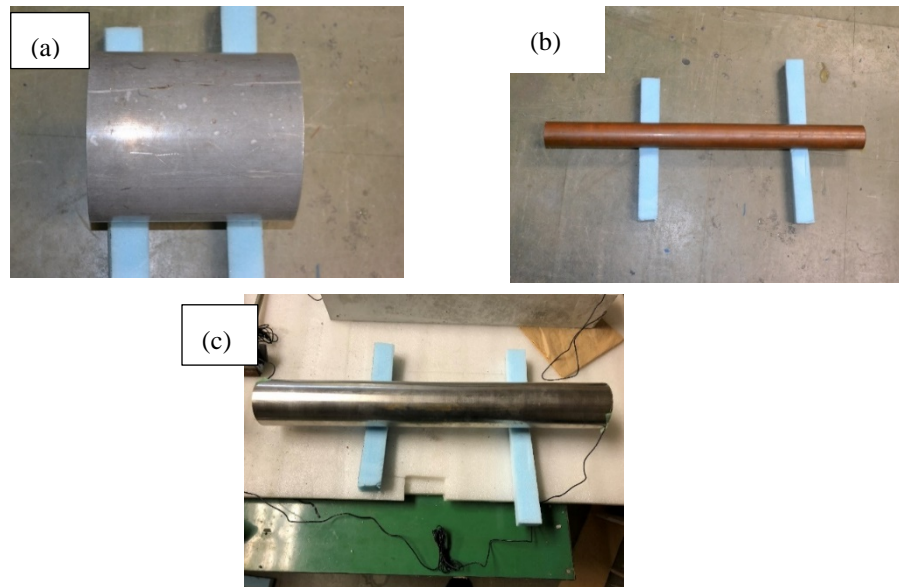
Figure 5. Setting of standard materials for EWV measurement, (a) Al, (b) Cu and (c) austenitic stainless steel (SUS304).
