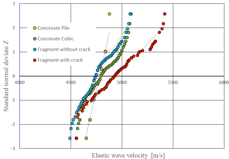
Figure 10. Cumulative distribution of EWV data of concrete
