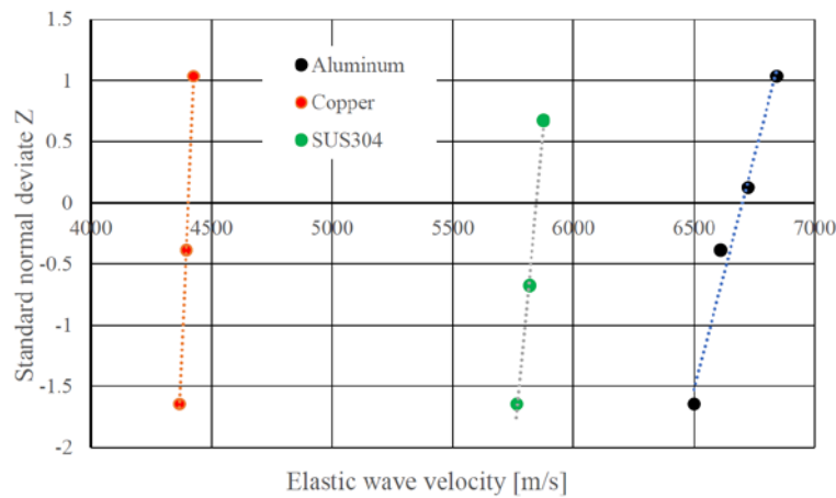
Figure 9. Cumulative distribution of EWV data of metals
