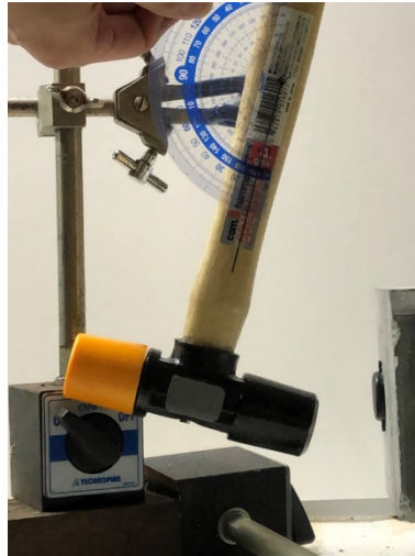
Figure 3. Alignment of the hammer impact method
