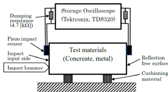
Figure 2. Measurement system for elastic wave velocity of concrete
