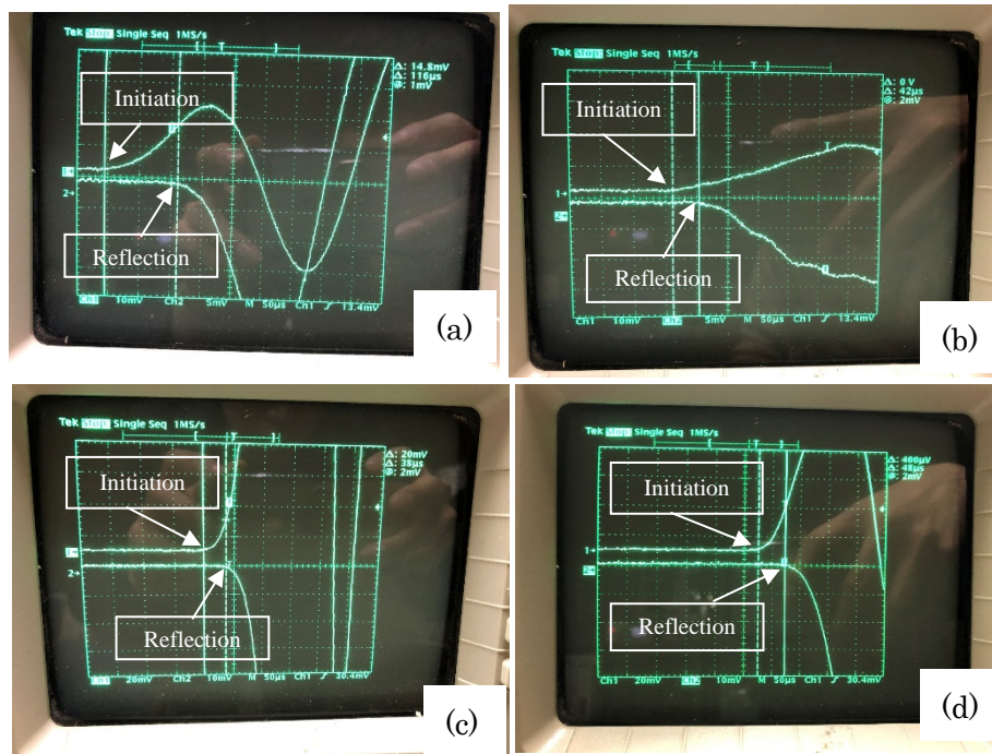
Figure 8 Elastic wave propagations of concrete on oscilloscope, (a) concrete pile having dimensions of 100×100×600 mm 3 , (b) concrete cube having dimensions of 200×200×200 mm 3 , (c) crashed concrete having no cracks, (d) crashed concrete with cracks. Time (a)~(d) 50μs/div.
