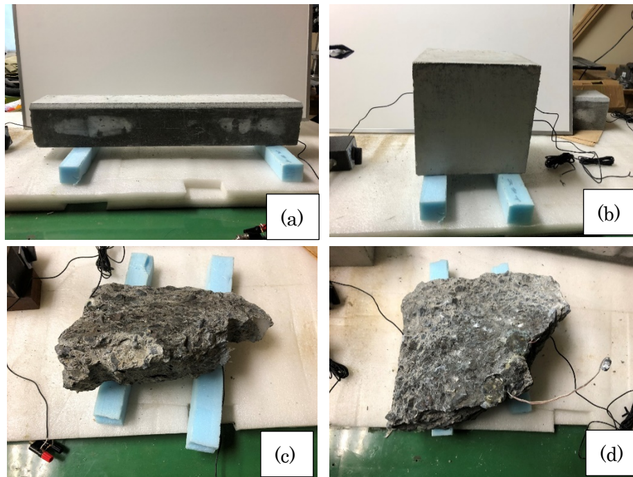
Figure 6. Concrete test pieces for EWV measurement, (a) pile of 100×100×600 mm 3 , (b) cube of 200×200×200 mm 3 , (c) crushed piece having approximately 400 mm length without cracks, (d) crushed piece having approximately 300 mm length with cracks.
