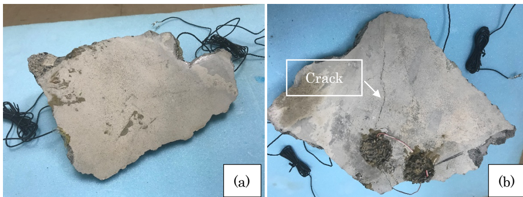
Figure 7. Concrete test pieces crashed by the steam pressure cracking agent, (a) piece having approximately 300 mm length without cracks, (b) piece having approximately 400 mm length with cracks.
