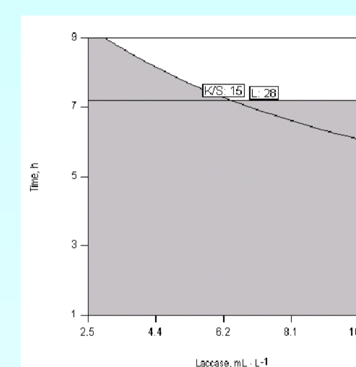
Figure 6 The optimum region defined by the overlaid plots of the two responses K/S and L* evaluated for modifier resorcinol as a function of laccase concentration and reaction time. The other factor was kept in the zero level
