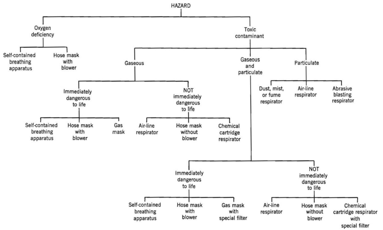
Figure 1. - Outline for selecting respiratory protective devices.
