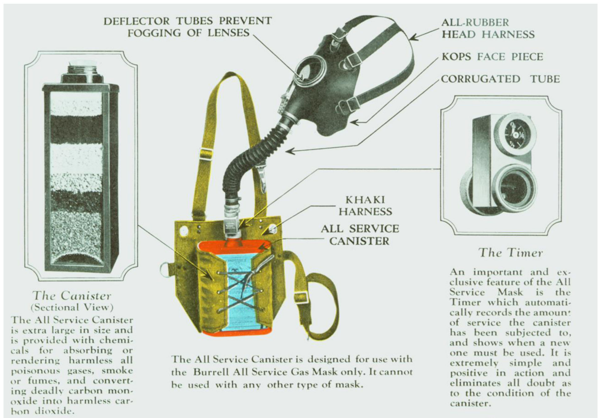
Figure 3. MSA Burrell All Purpose Gas Mask.
