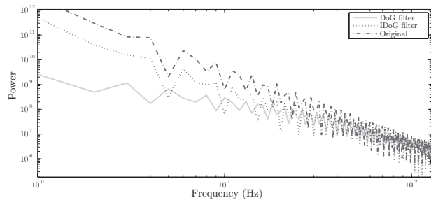
Figure 3. Power spectrum of an original frame (black square over a white background, slope equal to -2.87), as well as the frame output of the Lamina layer when using an IDoG (slope equal to -2.26) and a DoG (slope equal to -1.54) spatial filters, averaged over all orientations.
