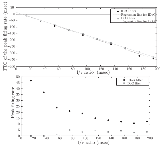
Figure 4. Top: Dependence of peak firing time relative to collision on l/|v| ratio obtained with the LGMD model, using a DoG filter as a model for the Lamina processing step (gray squares) and using an IDoG filter (black dots). Bottom: Relation between the peak firing rate obtained in the output of the LGMD cell and the l/|v| ratio.
