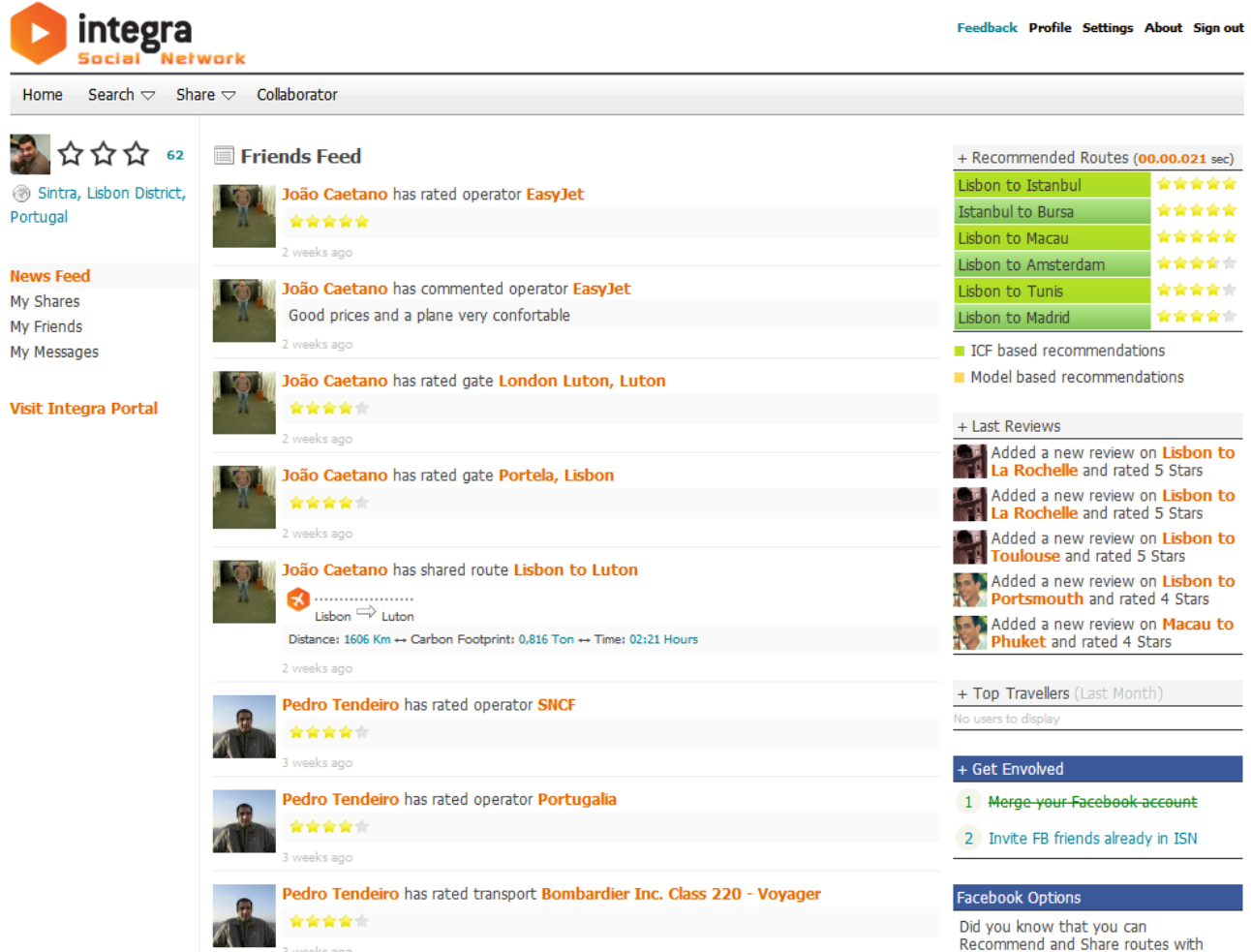
Figure 3. SMA application screen (Integra Social Network).
