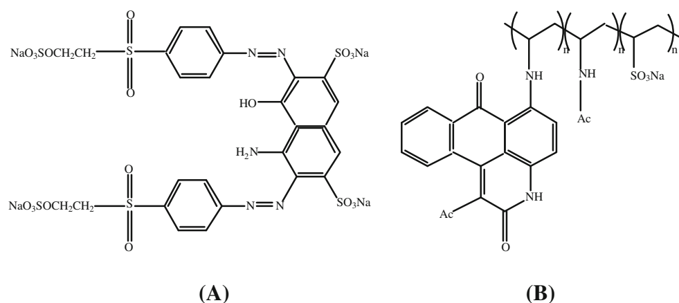
Fig. 1 Chemical structure of dyes used in this study: a RB5 and b Poly R-478
