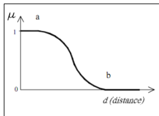
Figure 3: Fuzzy set membership function S-shaped
