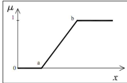
Figure 2: fuzzy set membership function (Linear)
