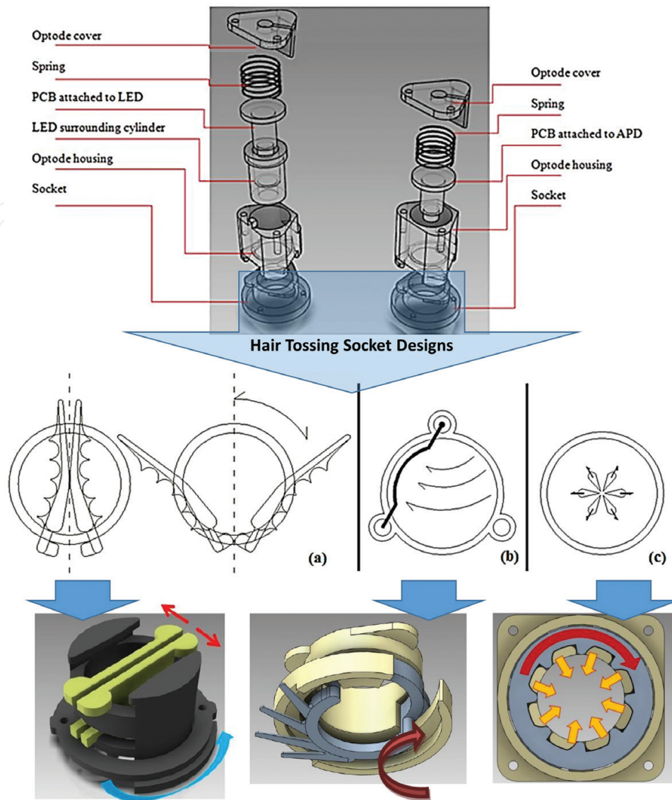
Figure 8. The various components of the optode housing and how it connects to the socket that is attached to the cap, a spring located inside the optode housing provides an additional pressure to maintain optode/scale contact. Hair clearing can be achieved via the development of socket designs that can play a dual role, by adding a hair clearing mechanism to it. Possible hair parting methods are: (a) dual parting pins, (b) single parting pin and (c) multiple parting [48].
