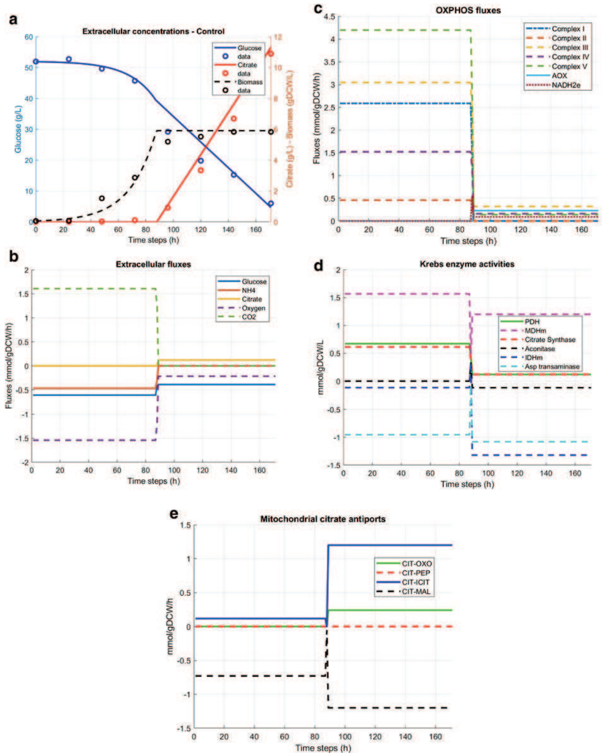
Figure 2. (a) Calibrating dFBA model with experimental flux rates allowed predictions close to experimental results, except for isocitrate which is not predicted by the model. (b) Simulated extracellular fluxes. Upon \text{NH}_4^+ limitation between 80 and 90 h, citrate flux increases. Glucose and oxygen consumption fluxes are lower during stationary phase (stat-phase). No \text{CO}_2 production is predicted at stat-phase. (c) Simulated oxidative phosphorylation (OXPHOS) activity. OXPHOS activity is globally reduced upon stat-phase. AOX and NADH2e are inhibited on growth phase and activated during stat-phase. Complexes I is inhibited on stat-phase, which is a marker of a the metabolic switch, with limited energy demand and activation of the alternative respiration through NADH2e-AOX axes. (d) Characterization of Krebs enzymes activities. On growth phase, Krebs cycle is active since pyruvate dehydrogenase (PDH), citrate synthase (CS), aconitase 1 and 2, mitochondrial isocitrate dehydrogenase (ISDHm) and malate dehydrogenase (MDHm) have positive fluxes. During stat-phase carbon fluxes are redirected towards mitochondrial citrate accumulation. Citrate-phosphoenolpyruvate (CIT-PEP) is inactive on both phases. Citrate-oxoglutarate (CIT-OXO) is active during stat-phase only. Both citrate-isocitrate (CIT-ICIT) and citrate-malate (CIT-MAL) increase their fluxes from growth to stat-phase.
