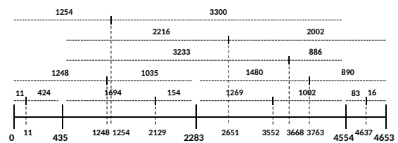
Fig. 1. Possible solution to the RNA PDP for the example considered. The primary cleavage sites (elements of \mathcal{P}_1 ) are represented by vertical solid lines while the secondary ones (elements of \mathcal{P}_2 ) by vertical dashed lines.
