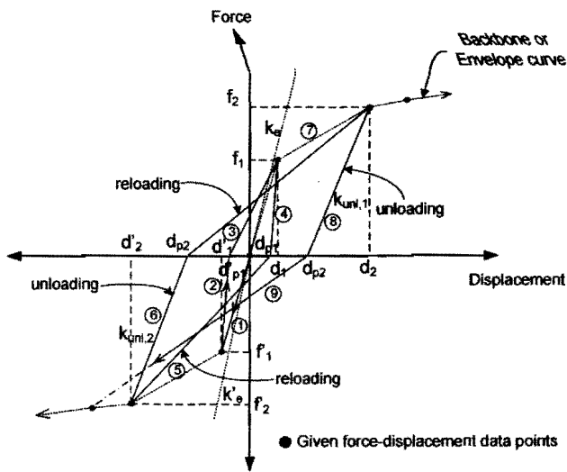
Figure 13 Modified Takeda hysteretic model
