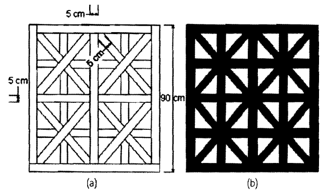
Figure 4 Configuration of the specimen: (a) dimensions; (b) location of the nails driven into the wood
