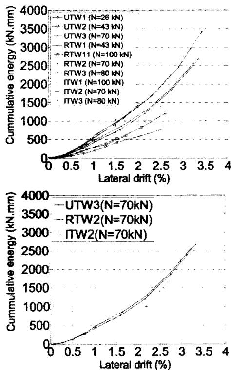
Figure 8 Cumulative energy dissipated by wall specimens vs. lateral drift
