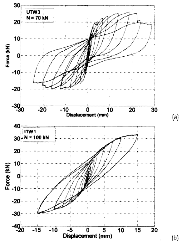
Figure 12 Load-displacement curves for (a) UTW3 and (b) ITW1
