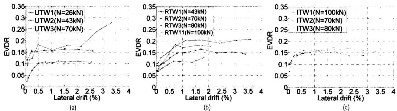
Figure 10 Equivalent viscous damping for (a) UTW, (b) RTW and (c) ITW
