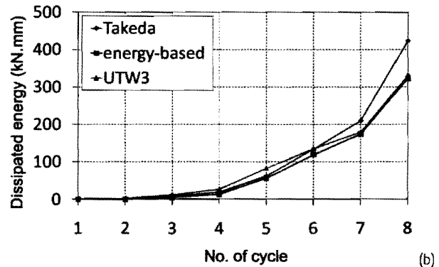
Figure 14 (a) Hysteretic model of UTW3 without pinching and (b) cyclic dissipated energy
