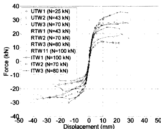
Figure 7 Envelope curves of wall specimens
