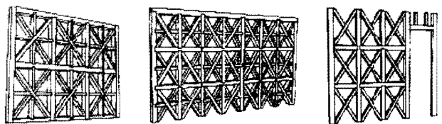
Figure 2 Different wall geometries in Pombalino buildings (Cóias 2007)
