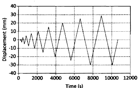
Figure 6 Typical cyclic displacement schedule
