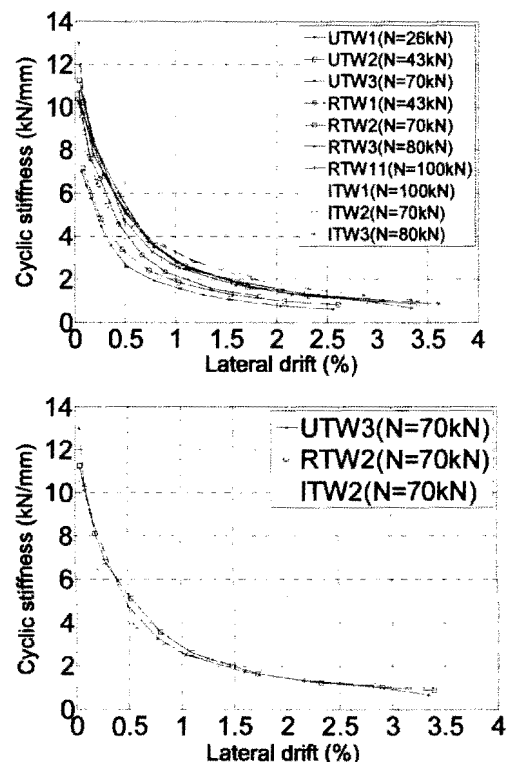
Figure 9 Overall cyclic stiffness of the wall vs. lateral drift
