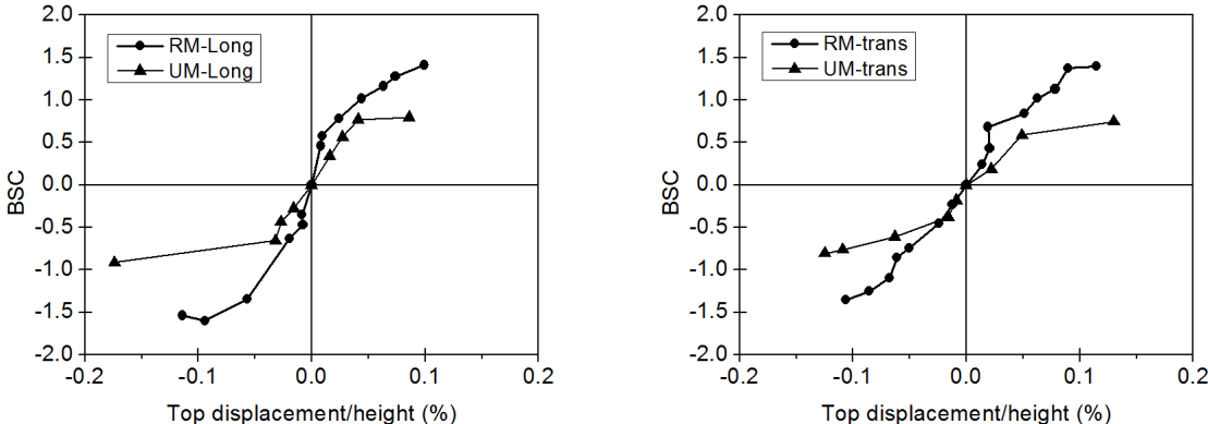
Figure 5. Hysteresis envelopes
