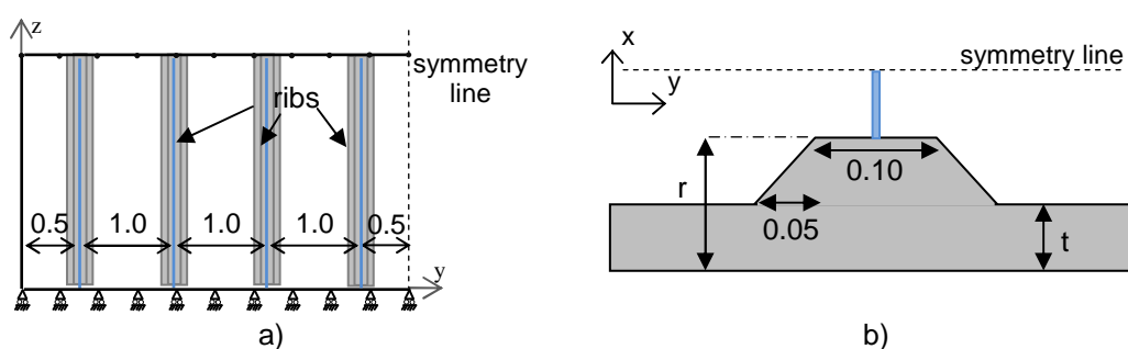
Figure 7: Sandwich panels comprising ribbed SFRSCC layers a) arrangement of ribs and connectors SFRSCC layers; b) detail of ribbed section (units in metres)
