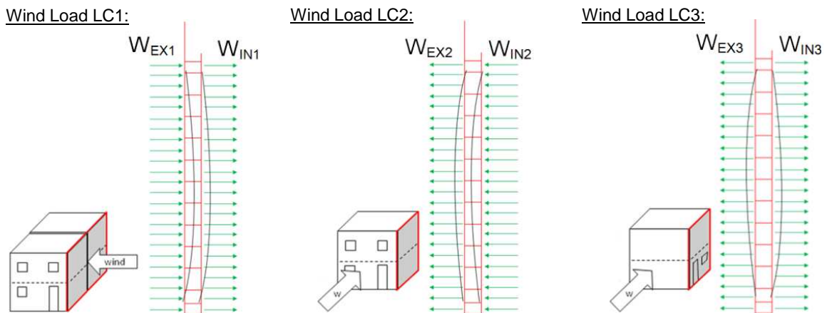
Figure 3: Wind load cases
