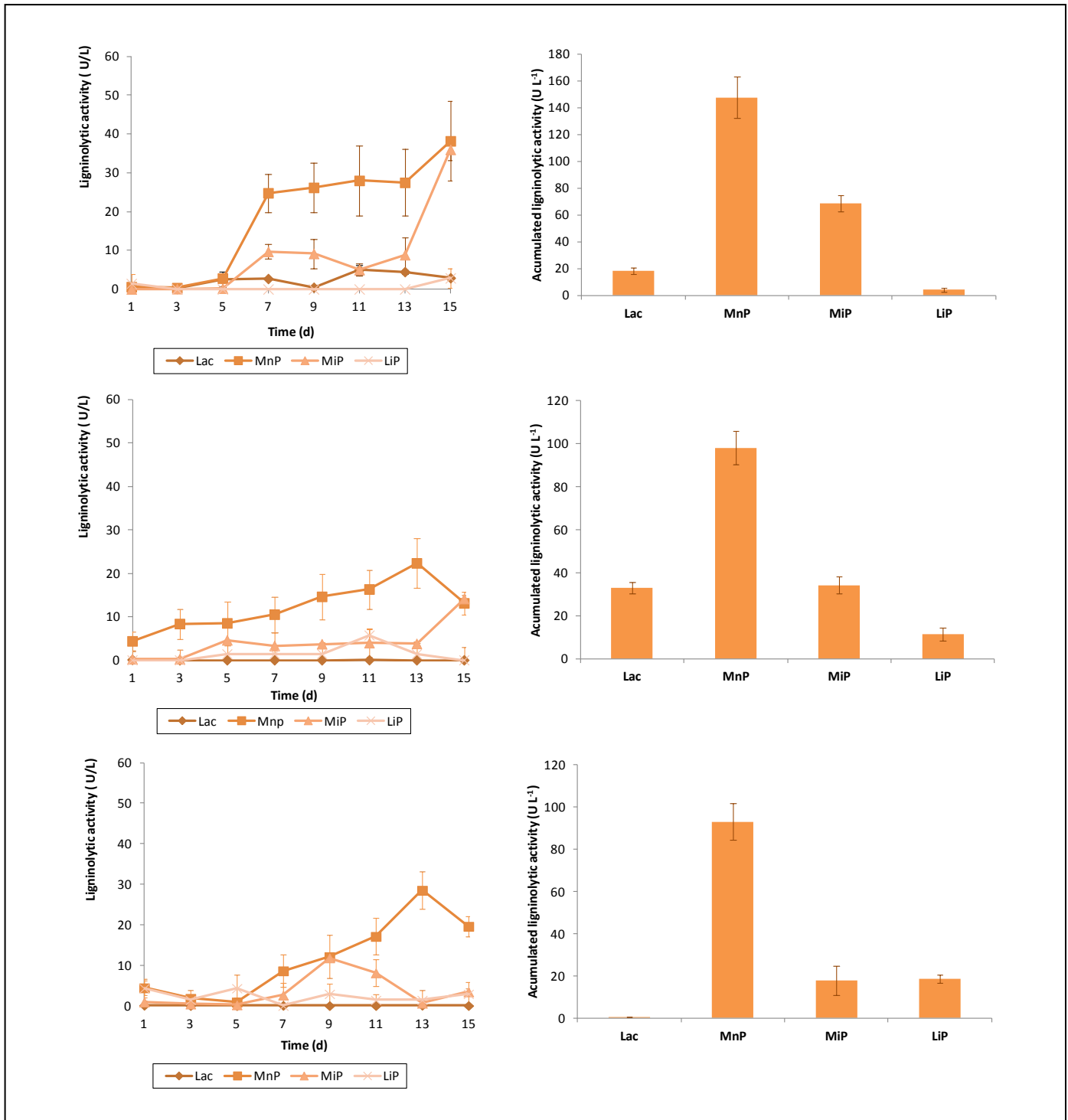
Fig. 5 Ligninolytic enzyme activities (left) and accumulated ligninolytic activity (right) of A. discolor pellets in liquid medium after 15 days of incubation at 26°C. (a) Complex pellets; (b) Coated pellets; (c) Simple pellets.
