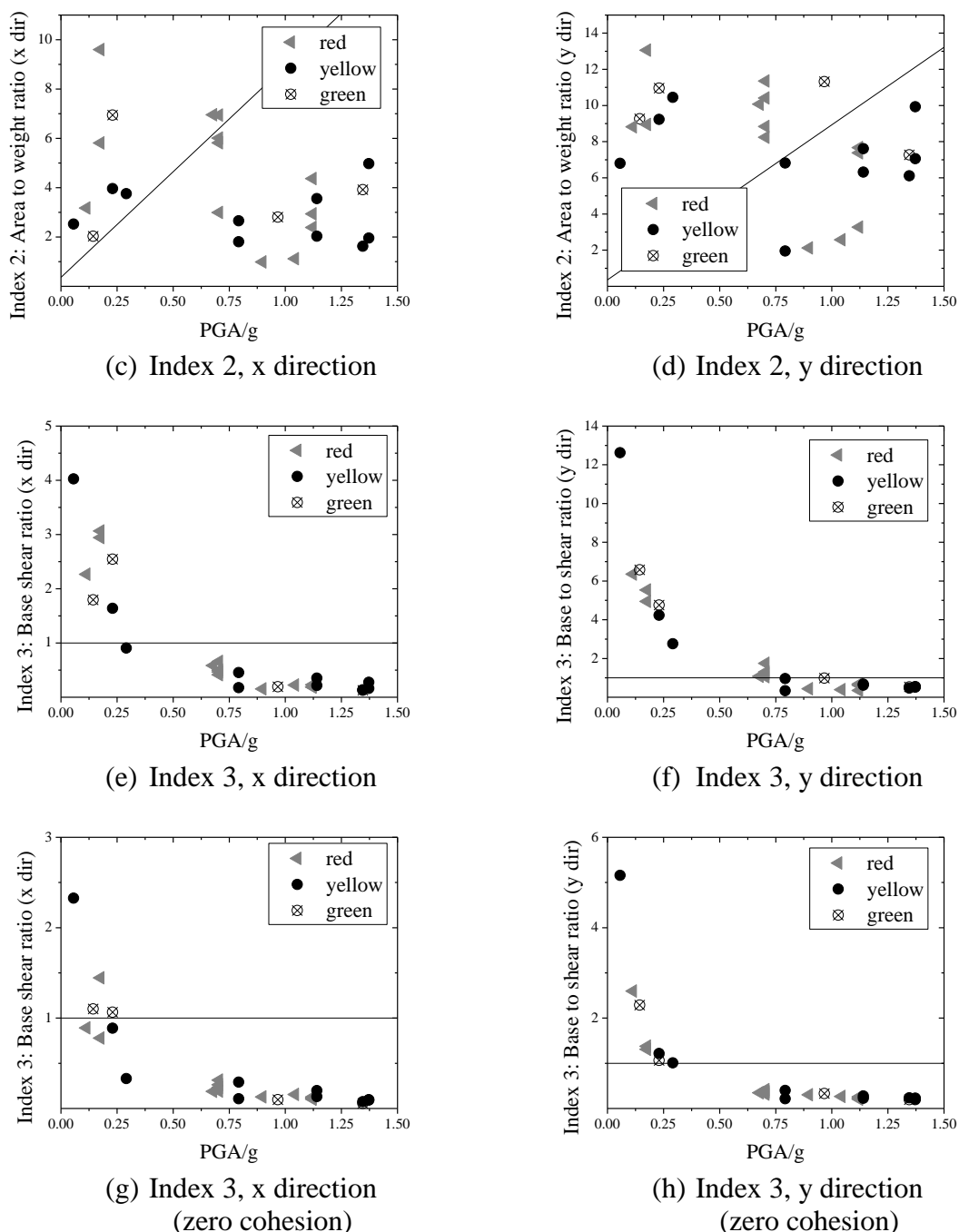
Figure 5. Indices for stone URM churches in the Canterbury earthquakes
