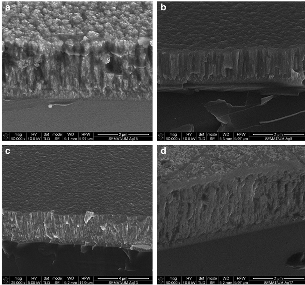
Fig. 4. Cross-sectional SEM micrographs for samples with atomic ratios Ag/Ti: a) 0; b) 0.20; c) 0.40 and d) 1.49.
