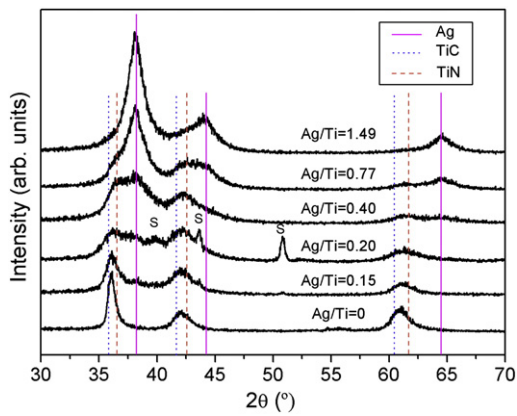
Fig. 1. XRD patterns of the Ag-TiCN coatings deposited by DC reactive magnetron sputtering, with different Ag/Ti atomic ratios.
