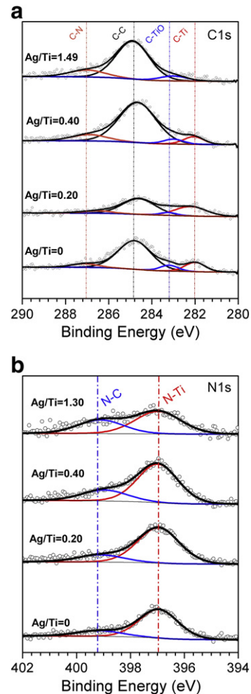
Fig. 2. C1s (a) and N1s (b) photoelectron spectra for 4 representative coatings with Ag/Ti ratios of 0, 0.20, 0.40 and 1.49.
