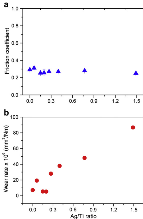
Fig. 7. Friction coefficient (a) and wear rate (b) values of Ag-TiCN as a function of the Ag/Ti atomic ratio.
