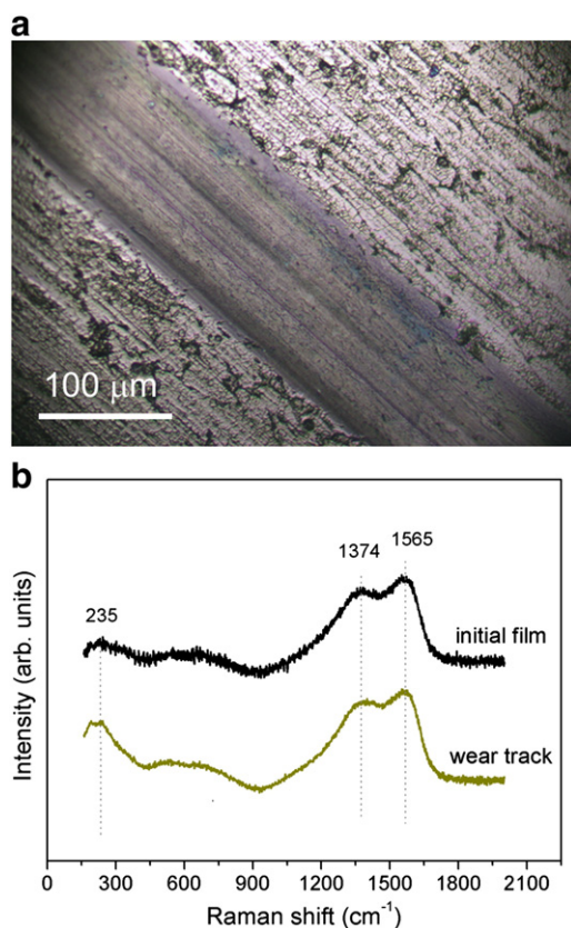
Fig. 9. Optical micrograph of the wear track after the friction test of the Ag-TiCN coating with 10.8 at.% of Ag (a) and corresponding Raman spectra (b).
