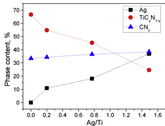
Fig. 3. Phase composition of the samples prepared with Ag/Ti ratios of 0, 0.20, 0.40 and 1.49.
