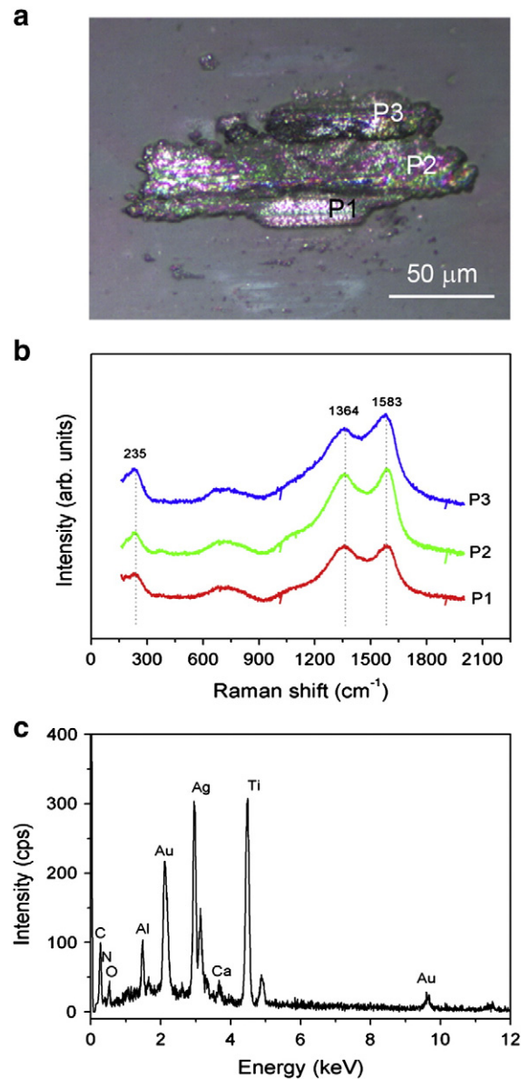
Fig. 8. Optical micrograph of the alumina ball after the friction test onto the Ag-TiCN coating with 10.8 at.% of Ag (a) and corresponding Raman spectra (b) and EDX (c) analysis.
