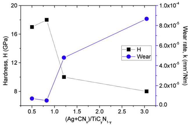
Fig. 6. Variation of the hardness and wear rate properties as a function of the ratio of soft (Ag + CN x )/hard (TiC y N 1-y ) phases.
