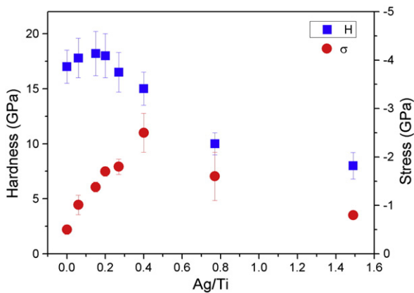
Fig. 5. Hardness and residual stress values of Ag-TiCN coatings vs. the Ag/Ti atomic ratio.
