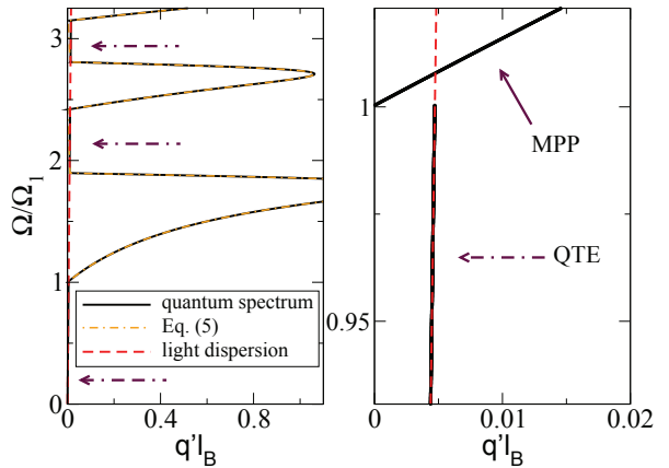
Figure 4: Mode spectrum for undoped graphene in a magnetic field ( N_F = 0 ) [solid (black) line]. We have taken \Gamma = 0.12E_1 in this figure. The light dispersion is shown in the dashed (red) line. Arrows in the left panel indicate the first three QTE modes.
