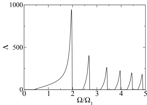
Figure 7: The wave localization ratio \Lambda is plotted as a function of the mode's frequency. Other parameters as in Fig. 1.
