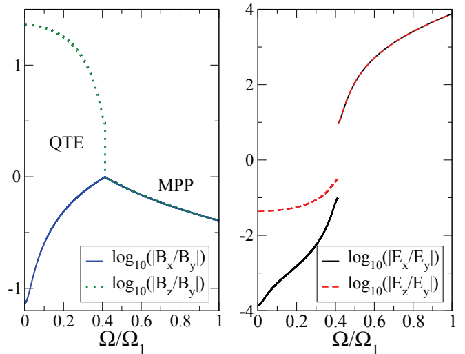
Figure 6: Polarization properties of the electromagnetic modes within the first two branches. The left panel shows the complex modulus of the magnetic ratios \mathcal{B}_{xy} and \mathcal{B}_{zy} , whereas the respective electric counterparts, \mathcal{E}_{xy} and \mathcal{E}_{zy} , are given in the right panel. (System parameters as in Fig. 1.)
