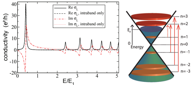
Figure 1: Doped graphene in a magnetic field at zero temperature ( N_F = 1 ). Left: \sigma_L is plotted as a function of E/E_1 , with E = \hbar\Omega and E_1 = E_1(B) . Clearly, \sigma_L'' < 0 in various energy intervals. The full quantum calculation is seen to be crucial for energies above \sim 2E_1 . We have taken \Gamma = 0.03E_1(B) , which, for B in the range 1-10 T, is consistent with experimental values of \Gamma (see text). Right: The first few electronic transitions are shown. The Fermi energy lies slightly above the Landau level with n = 1 , and thus only transitions to levels with n \geq 2 are allowed. The (small) dashed arrow stands for the intraband transition responsible for the strong peak observed near at (\sqrt{2} - 1)E_1 \sim 0.4E_1 . Other arrows represent interband transitions.
