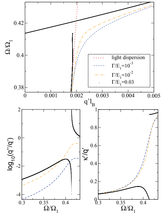
Figure 3: Mode spectrum and decay properties near a QTE-MPP transition. Top panel: The dispersion relation is plotted near at \Omega \simeq 0.4\Omega_1 for several broadening values (indicated in the legend). Bottom panel: The ratios q''(\Omega)/q'(\Omega) and \kappa'(\Omega)/q'(\Omega) are shown for the same parameter region in the top panel. For ease of visualization, the range for the vertical axis in left panel is limited. Other parameters as in Fig. 2.
