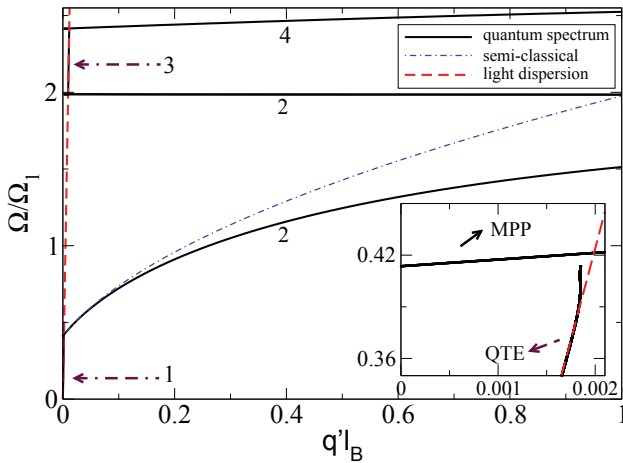
Figure 2: Mode frequency \Omega for graphene in vacuum is plotted as a function of the wave vector q' for doped graphene [solid (black) line]. The wave vector q' is given in units of the inverse of the magnetic length. For completeness, semi-classical solution [dashed-dotted (blue) line] and the light dispersion [dashed (red) line] are shown. Inset: Mode spectrum near at QTE-MPP transition at \Omega \simeq 0.4\Omega_1 . The numbers in the main panel identify the distinct branches up to \Omega \simeq 2.5\Omega_1 . For consistency with the local approximation to the conductivity, we have restricted our plots to the region with q'(\Omega)l_B \leq 1 . A considerable modification to the spectrum is expected for q' \sim l_B^{-1} due to non-local effects in the dynamical conductivity (see text). Other parameters as in Fig. 1.
