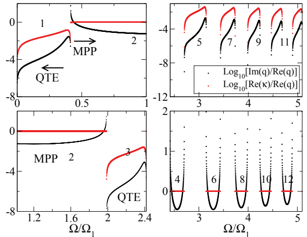
Figure 5: The ratios q''/q' and \kappa'/q' , which characterize the longitudinal and transverse decaying rates, respectively, are plotted in logarithmic scale as a function of the mode frequency. Several panels are given to help in visualizing the difference between QTE and MPP modes. (System parameters as in Fig. 1.)
