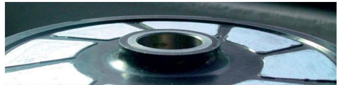
Fig. 4. Rotor of the AFIR-S Axial Flux motor used in the development of the methodology for parameters measurement [9].
