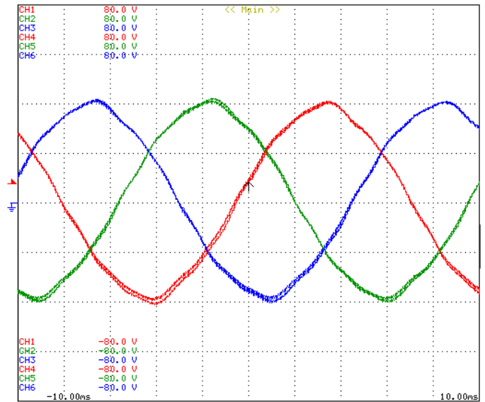
Fig. 8. Line-to-line voltages at the terminals of the two stators windings of the AFIR-S motor during the synchronization test.
