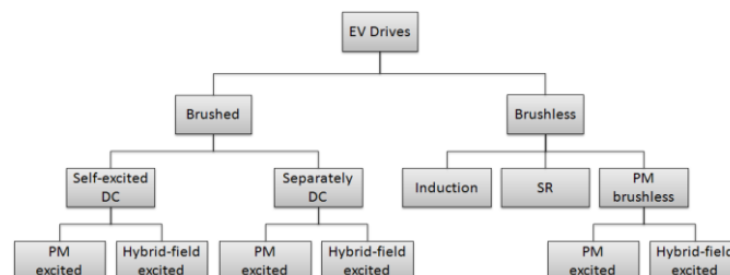
Fig. 1. Main types of electric motors used in electric vehicles [3].
