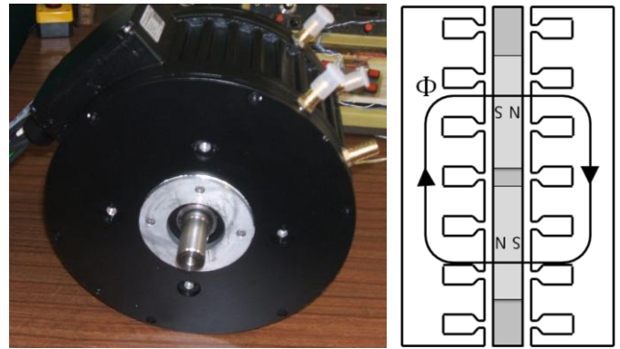
Fig. 3. AFIR-S Axial Flux Motor (on the left); Topology with flux direction (on the right) [6].
