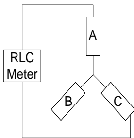
Fig. 9. Connection diagram to measure the synchronous inductance.
