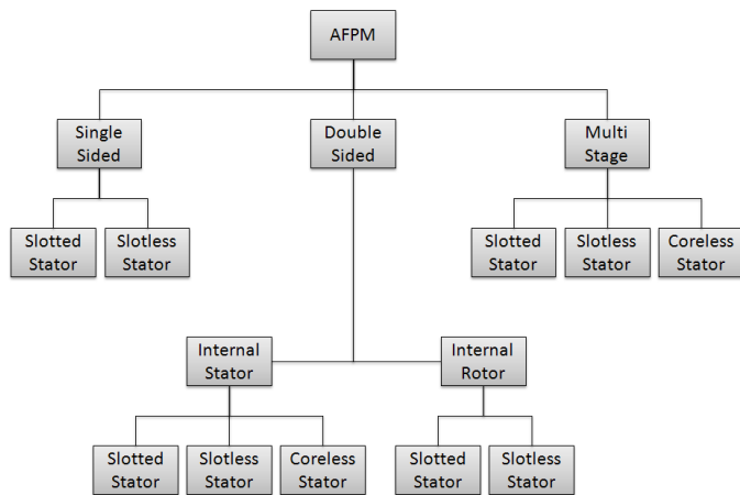
Fig. 2. Topologies of the Axial Flux Permanent Magnet (AFPM) motors.
