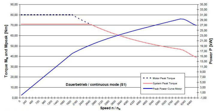
Fig. 5. Torque vs speed curve and power vs speed curve of the AFIR-S motor used in this study [9].
