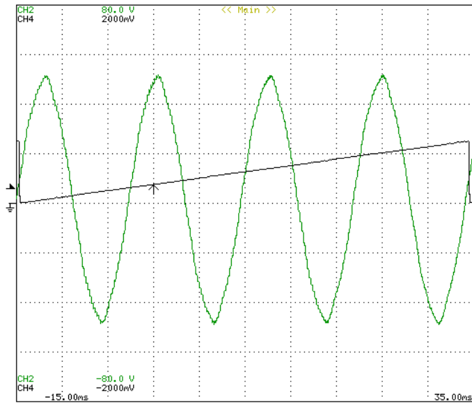
Fig. 11. Relation between the mechanical (black) and electrical (green) angle of the AFIR-S motor used in this study.
