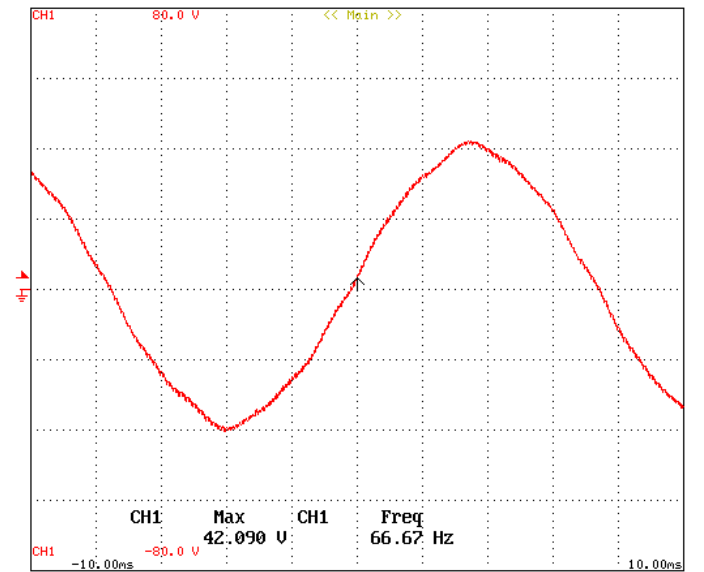
Fig. 10. Line-to-line voltage waveform when the motor operates as a generator without load at a speed of 1,000 rpm.
