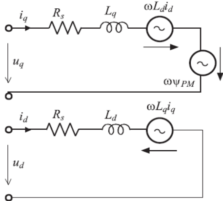
Fig. 6. Equivalent d - q model of the AFIR-S motor [11].
