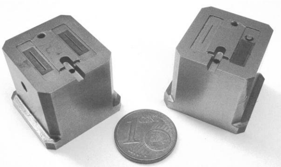
Figure 3 – Moulding blocks
