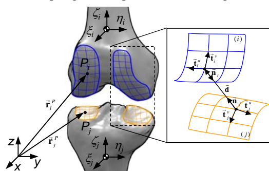
Figure 1: MBS knee model with contact surfaces.
