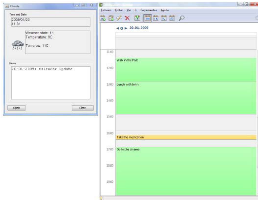
Fig. 3. Client Interface
