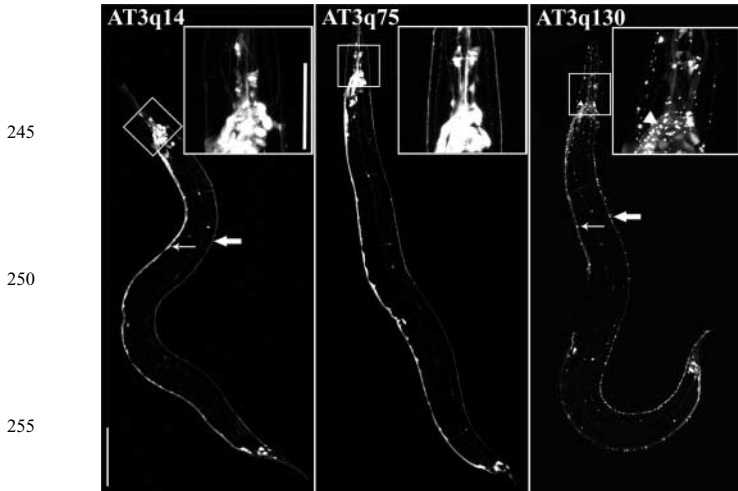
Figure 1. Pan-neuronal expression of full-length ATXN3 in C. elegans causes polyQ length-dependent changes in protein distribution. Expression of AT3q14 and AT3q75 proteins displayed a smooth and diffuse distribution pattern (left and middle panels, respectively), whereas AT3q130 proteins are found in discrete foci in certain neurons and are soluble in others (right panel). In the left panel, AT3q14 protein expression could be visualized in cell bodies (thin arrow) and in neuronal processes (thick arrow). In panel 3, the distribution of AT3q130 proteins was strikingly different: foci formation was clearly evident in VNC (thin arrow), DNC (thick arrow) and in certain cells of the circumpharyngeal nerve ring (arrow head). All animals depicted are young adults (4 days post-hatching). Scale bar, 100 \mu m. White boxes indicate magnified regions. The images were obtained using a Zeiss LSM 510 confocal microscope.
