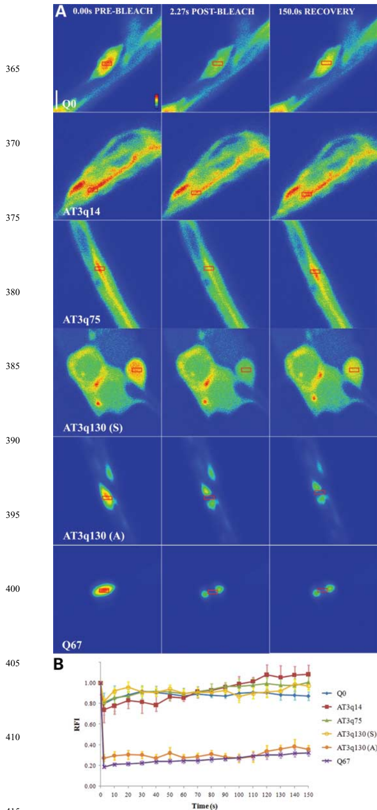
Figure 2. Expression of full-length ATXN3 in live neuronal cells causes polyQ length-dependent aggregation. For FRAP of neurons expressing Q0 proteins, the RFI of the photobleached area (red box), recovers rapidly (A and B ‘Q0’). Similar results were obtained in neurons expressing WT AT3q14 and AT3q75 (A and B ‘AT3q14’ and ‘AT3q75’), indicating the
