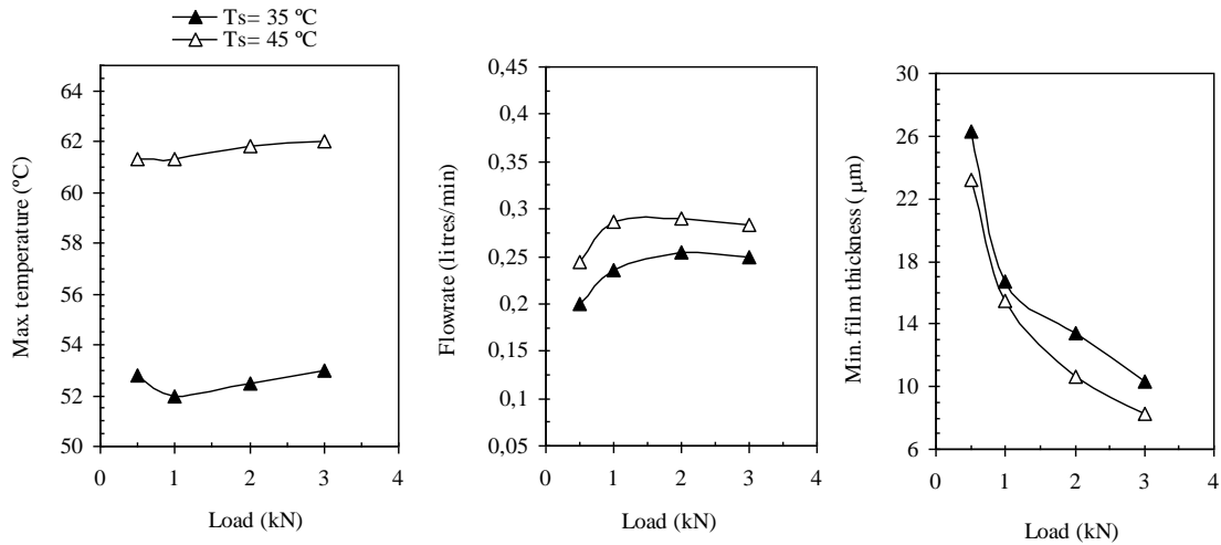
Figure 8- Measured performance characteristics of bearing C for variable oil supply temperature, at fixed P_s = 100 kPa and N = 3000 rpm
