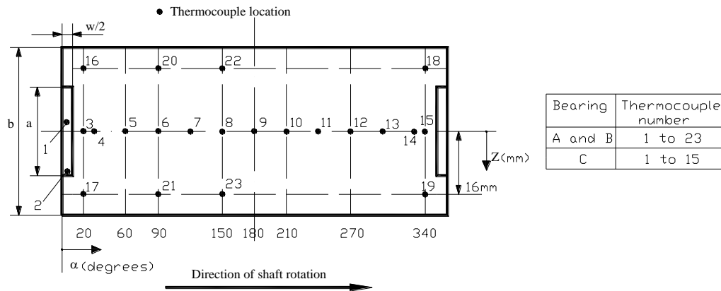
Figure 3- Location of thermocouples for temperature measurements
