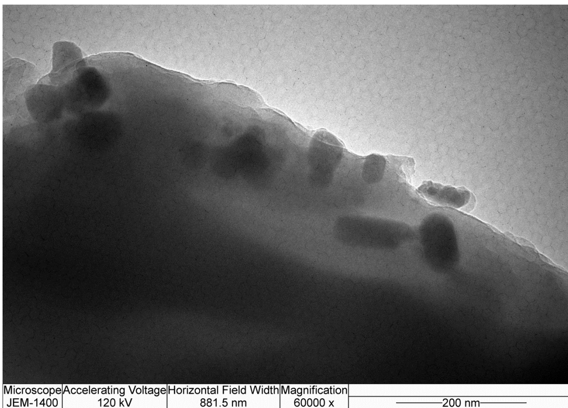
Fig. 11. TEM micrograph of the 6MZF-P_PVA20+PEG6 .
