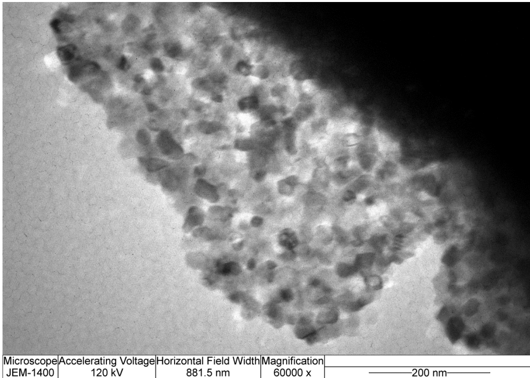
Fig. 10. TEM micrograph of the 4MZF-B_PVA2+PEG06 .
