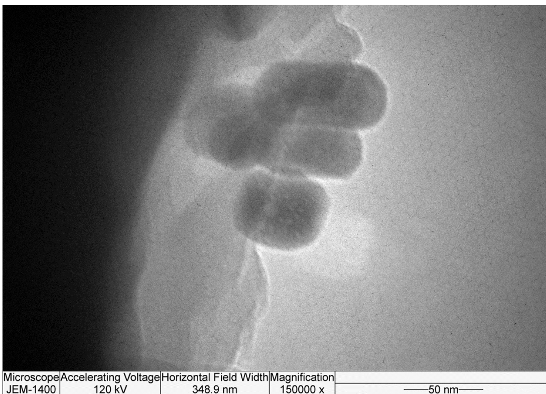
Fig. 12. TEM micrograph of the 6MZF-P_PVA20+PEG6 .
