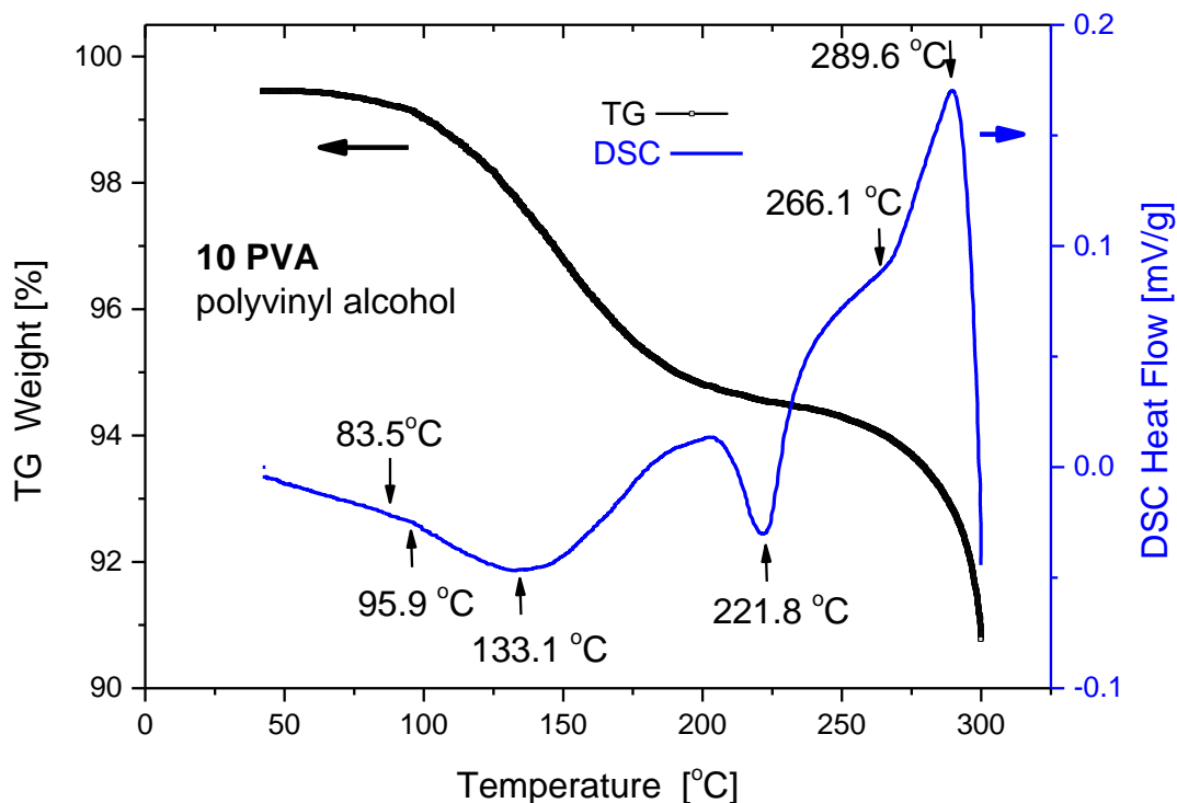
Fig.2. TG/DTA diagram of PVA - Poly vinyl alcohol, 10 PVA .
