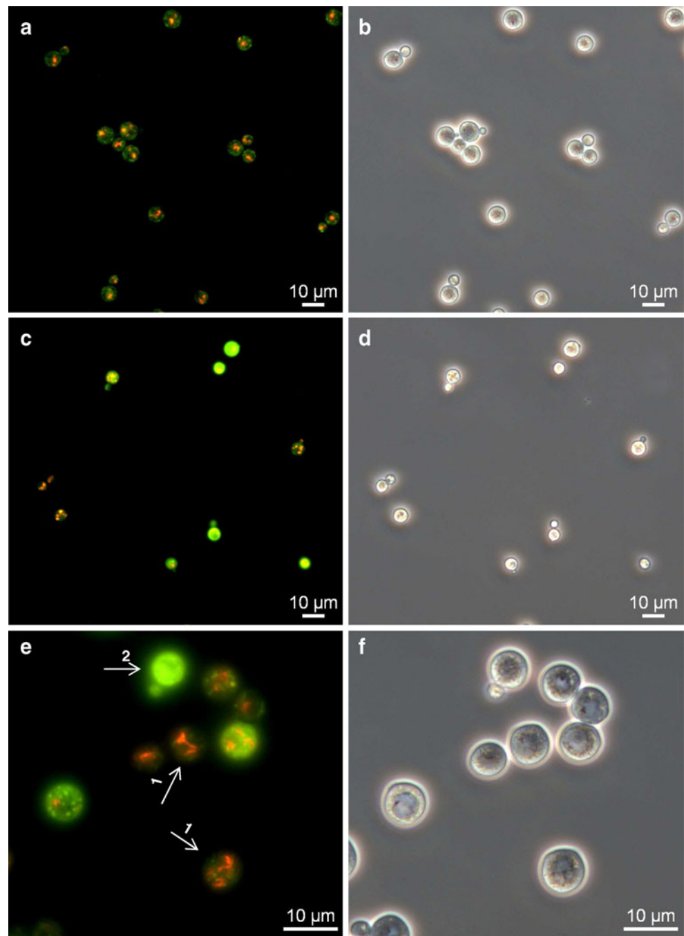
Fig. 4 Cells of S. cerevisiae NCYC 1214 stained with FUN-1. Fluorescence micrographs ( a , c , and e ); phase contrast micrographs of the same cells ( b , d , and f ). Micrographs of cells before being exposed ( a and b ) or after being exposed, during 2 h to 1,000 \mu\text{mol/l} \text{Pb}(\text{NO}_3)_2 ( c–f ). Arrow 1 : metabolic active cells with CIVS; arrow 2 : metabolic inactive cells (cells without CIVS)
