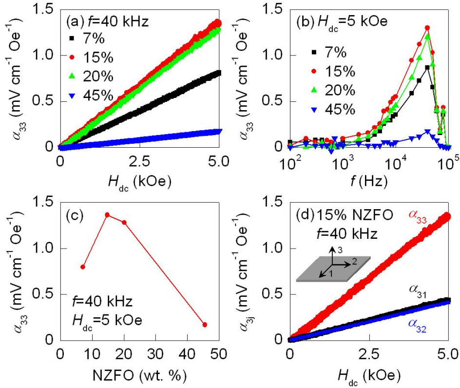
Figure 3. Room-temperature dynamic magnetolectric response of 50 \mu\text{m} -thick NZFO/P(VDF-TrFE) 0-3 nanocomposites to out-of-plane H_{\text{ac}} fields of magnitude 1.27 Oe. (a) Magnetolectric voltage coefficient \alpha_{33} as a function of H_{\text{dc}} at resonance and (b) as a function of frequency at H_{\text{dc}} = 5 kOe . (c) Maximum value of \alpha_{33} as a function of NZFO content. (d) \alpha_{3j} as a function of H_{\text{dc}} magnitude and direction (inset) at resonance for the sample with 15 wt. % NZFO. In (a) and (d), magnetolectric voltage is plotted for both increasing and decreasing H_{\text{dc}} .
