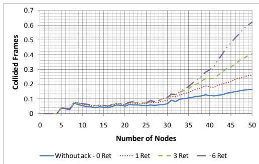
Figure 3. Collided packets curves
