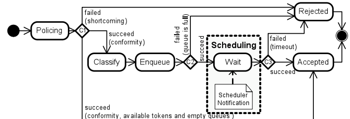
Figure 1. Admission Control Scheme
