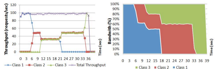
Figure 3. MCF results
