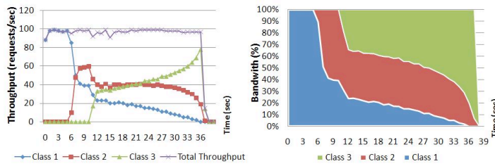
Figure 4. CBFQ results
