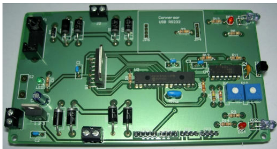
Figure 19. Board with components soldered
