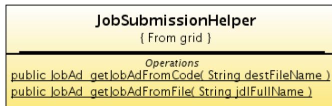
Figure 7-3: JobSubmissionHelper class
