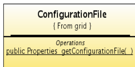
Figure 7-4: ConfigurationFile class
