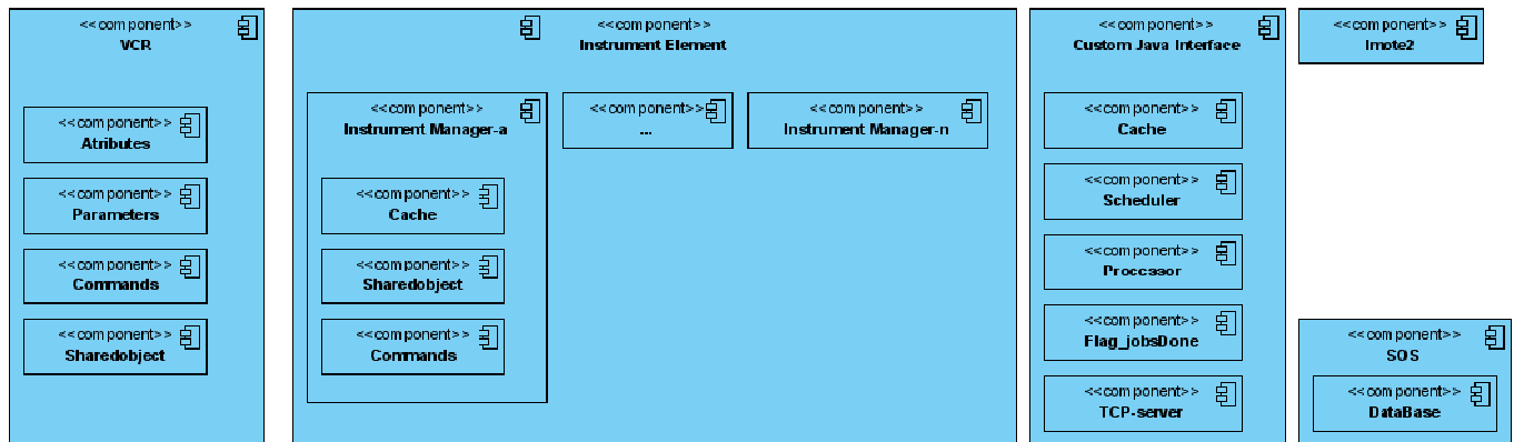
Figure 8-4: The software components of the architecture used to integrate a WSN into the Grid
