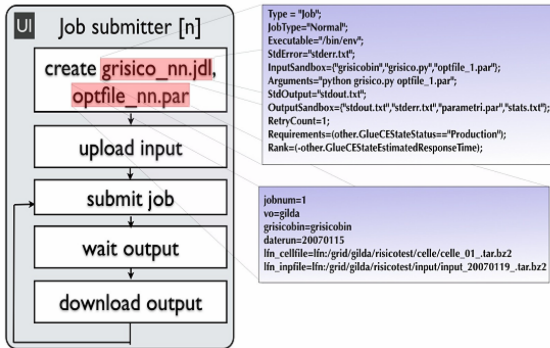
Figure 6-3: the job submitter component schema
