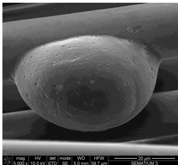
Fig. 6. SEM micrograph of GF/PP towpreg (magnification of 5000x).
