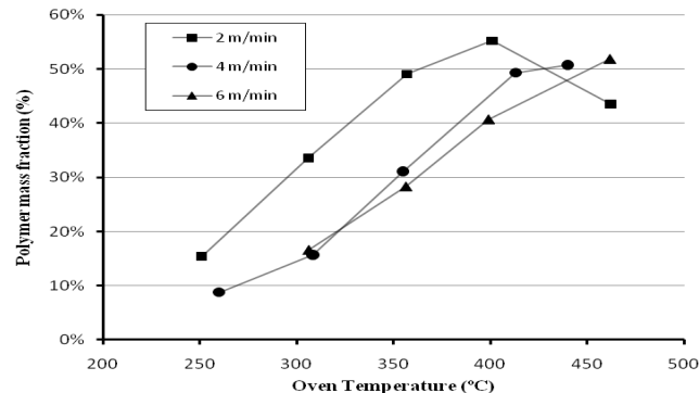
Fig. 2. Variation of the polymer mass fraction with oven temperature and fibre pull-speed
