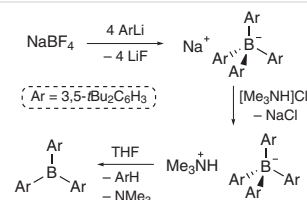
Scheme 1 Synthesis of B(3,5- t Bu 2 C 6 H 3 ) 3
